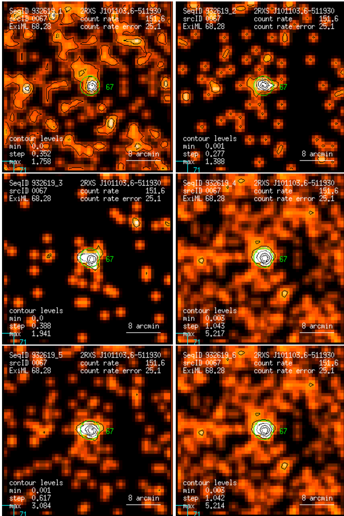
Figure 67: RASS 932619: detection 0067: band rate images, Gaussian filter: (1) PSPC channels 11 – 41, (2) 52 – 90, (3) 91 – 201, (4) 11 – 235, (5) 52 – 201, (6) 11 – 201. Broad band rates in counts/ks. Band rate contour levels in counts/ks/arcmin 2 .
