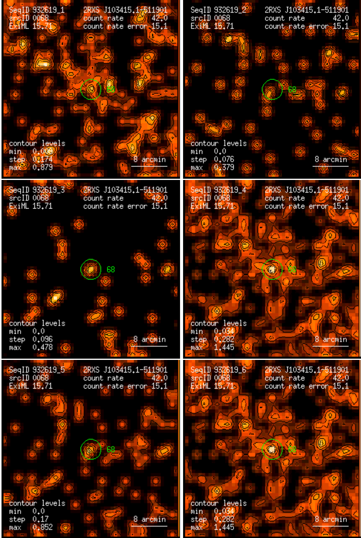
Figure 68: RASS 932619: detection 0068: band rate images, Gaussian filter: (1) PSPC channels 11 – 41, (2) 52 – 90, (3) 91 – 201, (4) 11 – 235, (5) 52 – 201, (6) 11 – 201. Broad band rates in counts/ks. Band rate contour levels in counts/ks/arcmin 2 .
