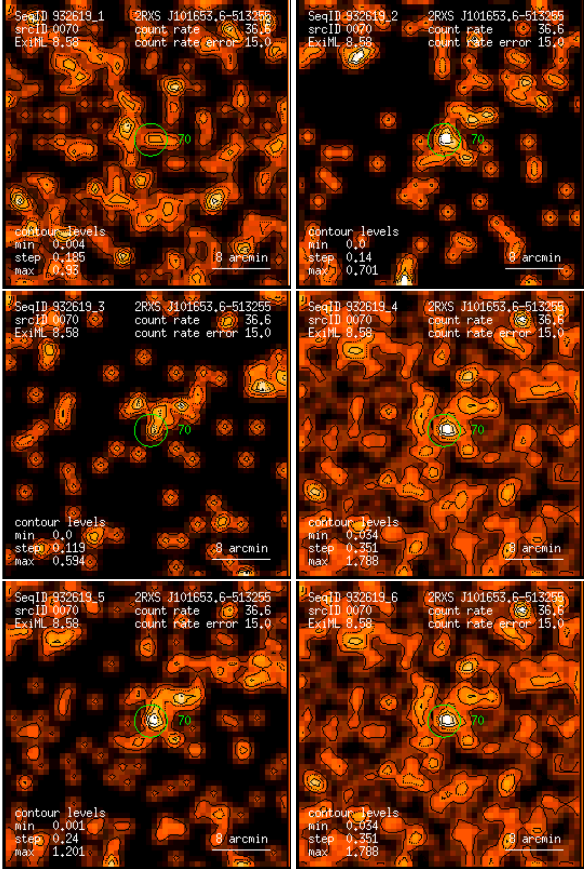
Figure 70: RASS 932619: detection 0070: band rate images, Gaussian filter: (1) PSPC channels 11 – 41, (2) 52 – 90, (3) 91 – 201, (4) 11 – 235, (5) 52 – 201, (6) 11 – 201. Broad band rates in counts/ks. Band rate contour levels in counts/ks/arcmin 2 .
