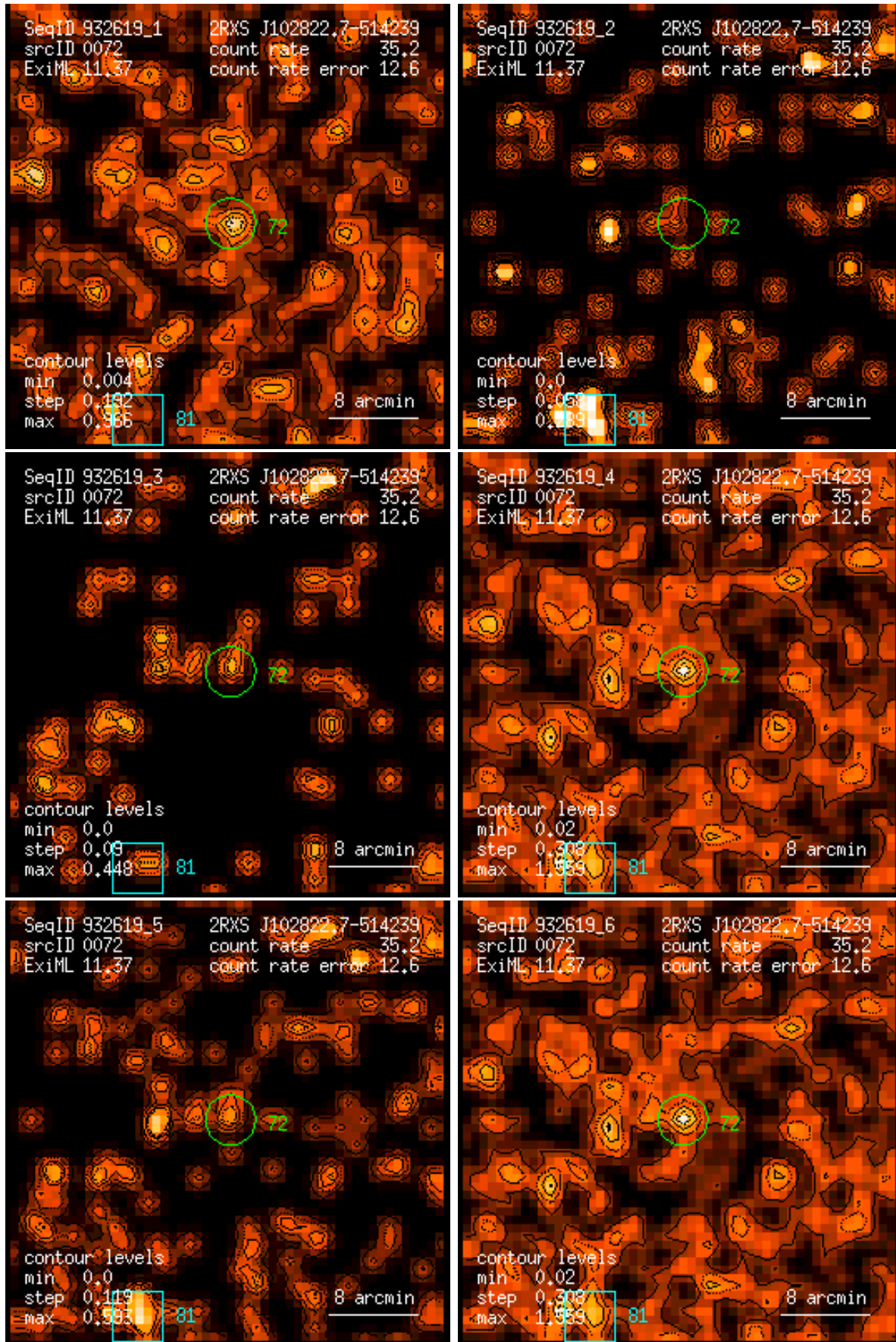
Figure 72: RASS 932619: detection 0072: band rate images, Gaussian filter: (1) PSPC channels 11 – 41, (2) 52 – 90, (3) 91 – 201, (4) 11 – 235, (5) 52 – 201, (6) 11 – 201. Broad band rates in counts/ks. Band rate contour levels in counts/ks/arcmin 2 .
