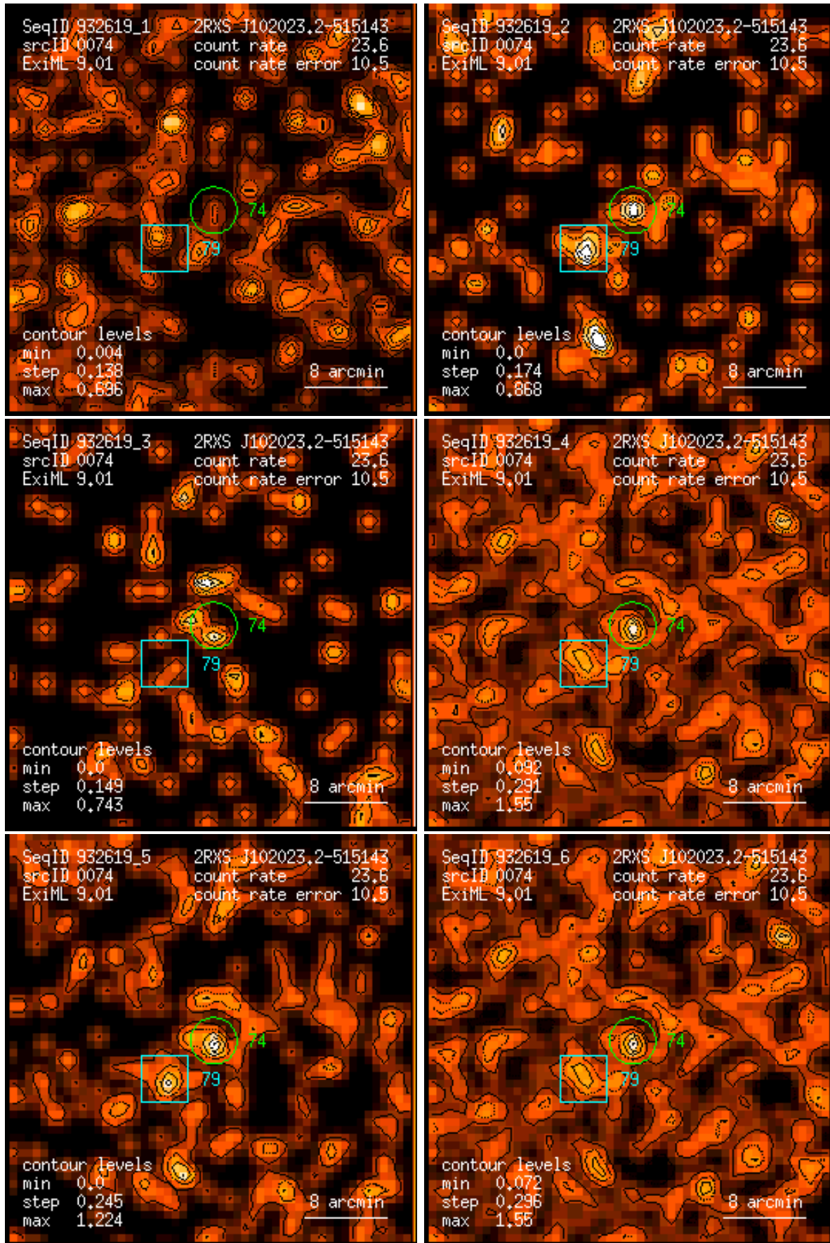
Figure 74: RASS 932619: detection 0074: band rate images, Gaussian filter: (1) PSPC channels 11 – 41, (2) 52 – 90, (3) 91 – 201, (4) 11 – 235, (5) 52 – 201, (6) 11 – 201. Broad band rates in counts/ks. Band rate contour levels in counts/ks/arcmin 2 .
