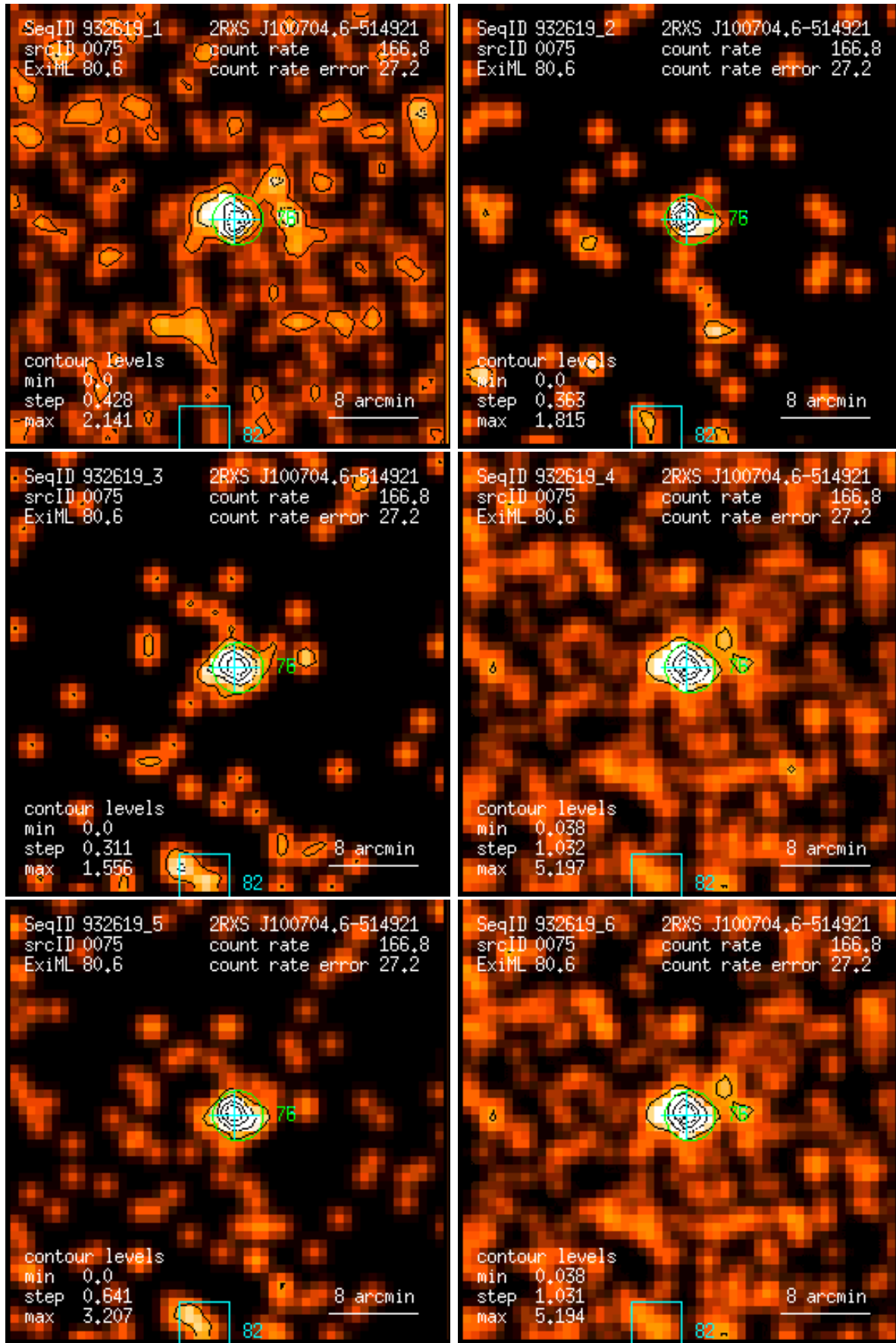
Figure 75: RASS 932619: detection 0075: band rate images, Gaussian filter: (1) PSPC channels 11 – 41, (2) 52 – 90, (3) 91 – 201, (4) 11 – 235, (5) 52 – 201, (6) 11 – 201. Broad band rates in counts/ks. Band rate contour levels in counts/ks/arcmin 2 .
