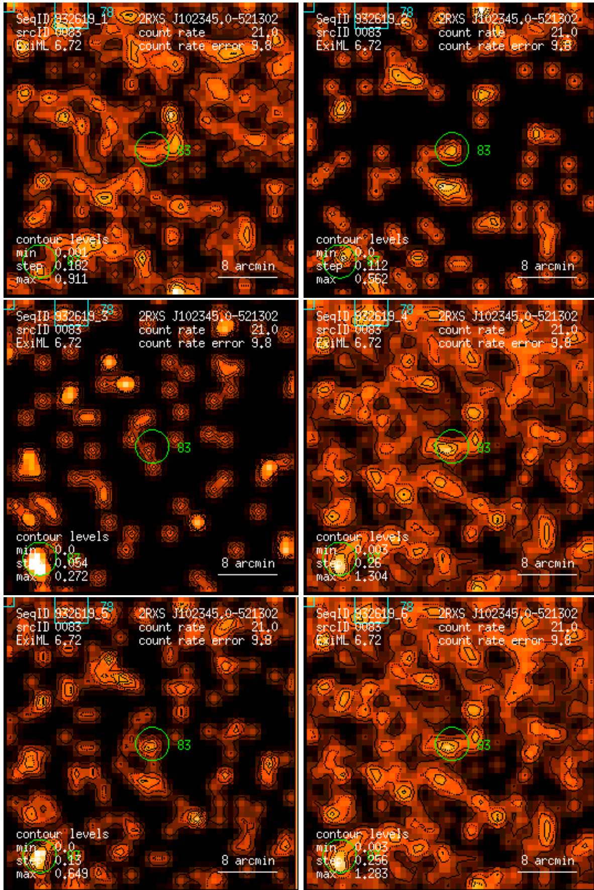
Figure 83: RASS 932619: detection 0083: band rate images, Gaussian filter: (1) PSPC channels 11 – 41, (2) 52 – 90, (3) 91 – 201, (4) 11 – 235, (5) 52 – 201, (6) 11 – 201. Broad band rates in counts/ks. Band rate contour levels in counts/ks/arcmin 2 .
