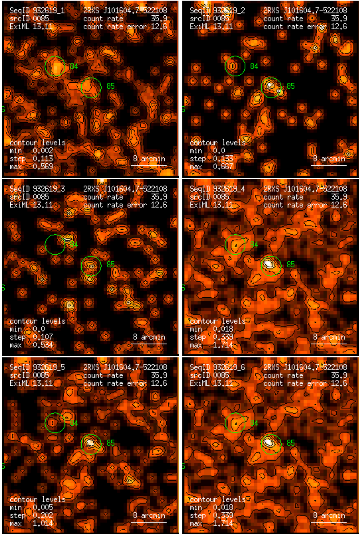
Figure 85: RASS 932619: detection 0085: band rate images, Gaussian filter: (1) PSPC channels 11 – 41, (2) 52 – 90, (3) 91 – 201, (4) 11 – 235, (5) 52 – 201, (6) 11 – 201. Broad band rates in counts/ks. Band rate contour levels in counts/ks/arcmin 2 .
