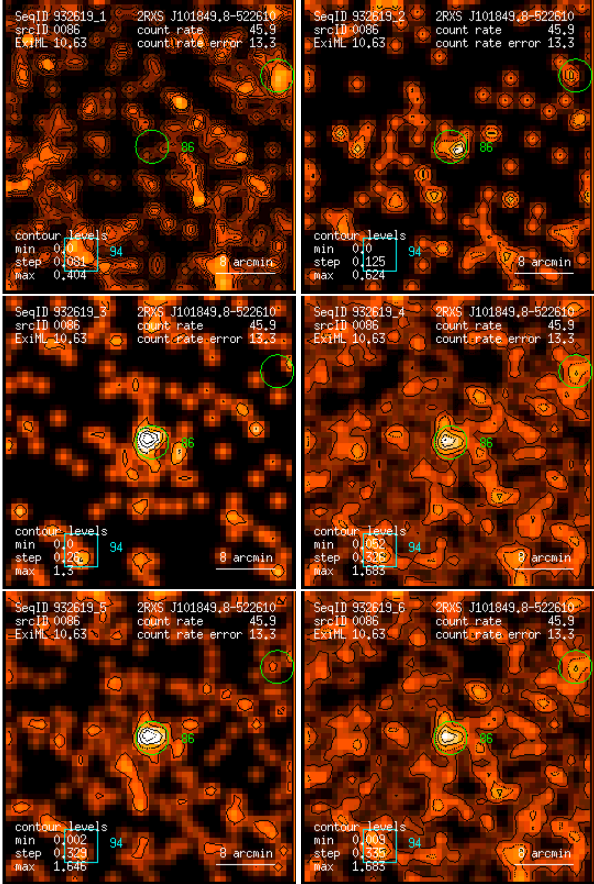
Figure 86: RASS 932619: detection 0086: band rate images, Gaussian filter: (1) PSPC channels 11 – 41, (2) 52 – 90, (3) 91 – 201, (4) 11 – 235, (5) 52 – 201, (6) 11 – 201. Broad band rates in counts/ks. Band rate contour levels in counts/ks/arcmin 2 .
