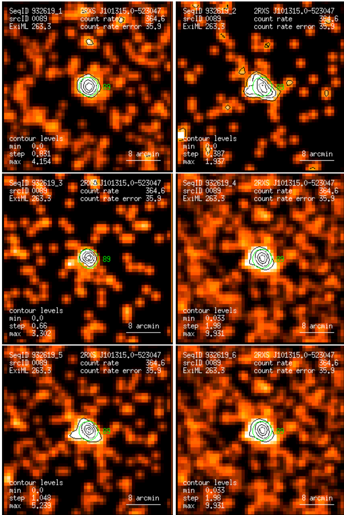
Figure 89: RASS 932619: detection 0089: band rate images, Gaussian filter: (1) PSPC channels 11 – 41, (2) 52 – 90, (3) 91 – 201, (4) 11 – 235, (5) 52 – 201, (6) 11 – 201. Broad band rates in counts/ks. Band rate contour levels in counts/ks/arcmin 2 .
