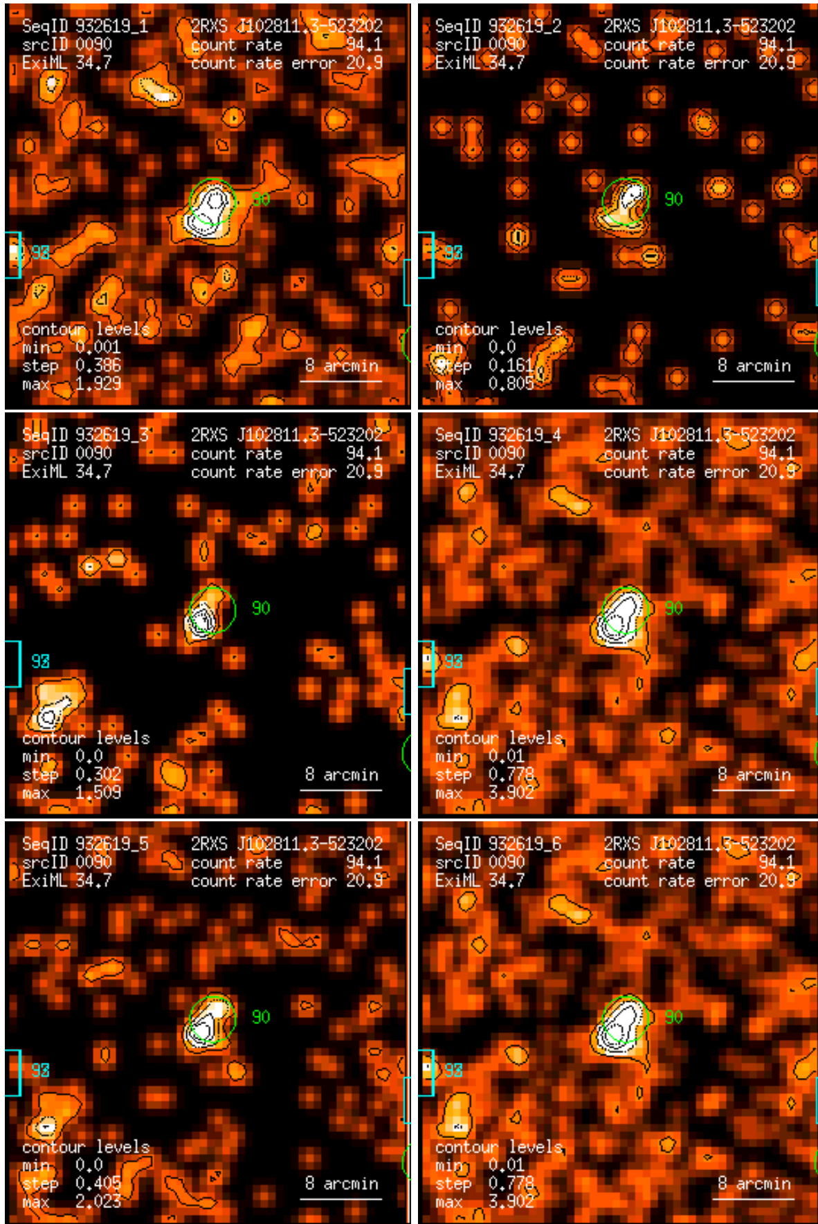
Figure 90: RASS 932619: detection 0090: band rate images, Gaussian filter: (1) PSPC channels 11 – 41, (2) 52 – 90, (3) 91 – 201, (4) 11 – 235, (5) 52 – 201, (6) 11 – 201. Broad band rates in counts/ks. Band rate contour levels in counts/ks/arcmin 2 .
