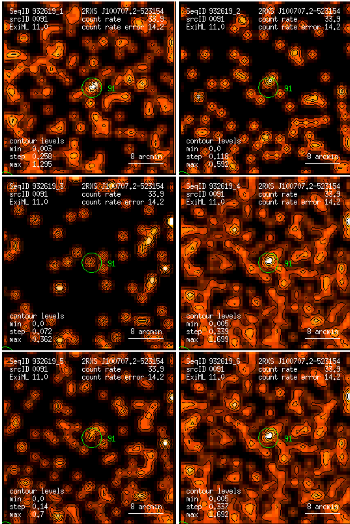
Figure 91: RASS 932619: detection 0091: band rate images, Gaussian filter: (1) PSPC channels 11 – 41, (2) 52 – 90, (3) 91 – 201, (4) 11 – 235, (5) 52 – 201, (6) 11 – 201. Broad band rates in counts/ks. Band rate contour levels in counts/ks/arcmin 2 .
