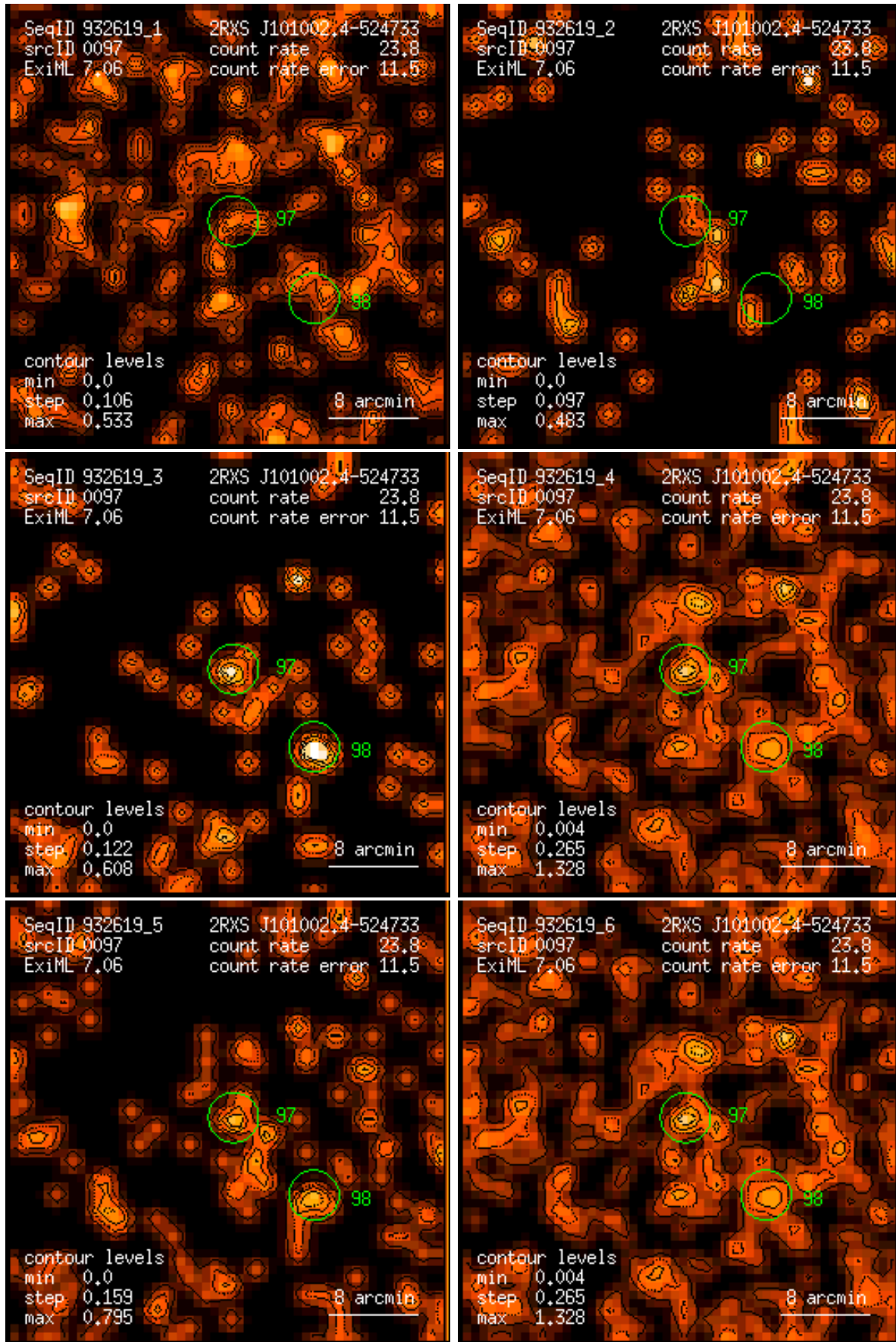
Figure 97: RASS 932619: detection 0097: band rate images, Gaussian filter: (1) PSPC channels 11 – 41, (2) 52 – 90, (3) 91 – 201, (4) 11 – 235, (5) 52 – 201, (6) 11 – 201. Broad band rates in counts/ks. Band rate contour levels in counts/ks/arcmin 2 .
