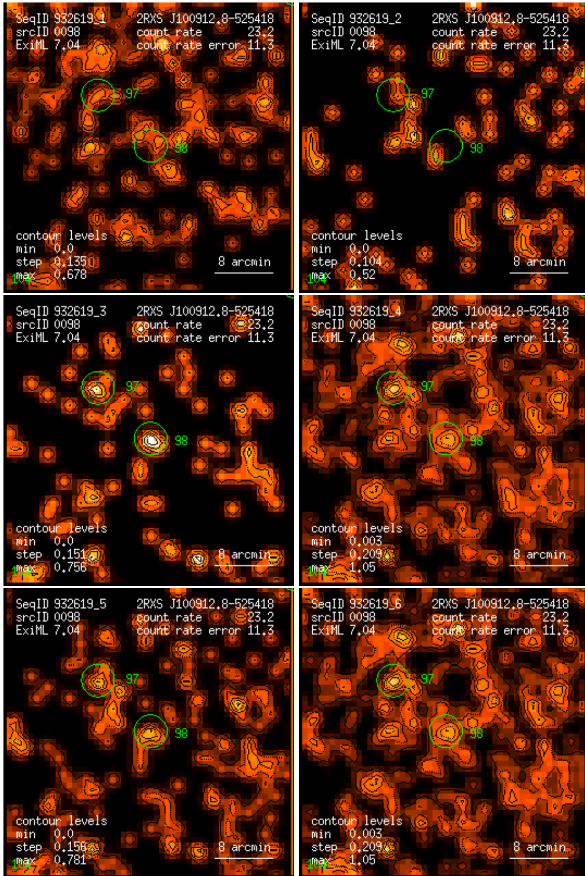
Figure 98: RASS 932619: detection 0098: band rate images, Gaussian filter: (1) PSPC channels 11 – 41, (2) 52 – 90, (3) 91 – 201, (4) 11 – 235, (5) 52 – 201, (6) 11 – 201. Broad band rates in counts/ks. Band rate contour levels in counts/ks/arcmin 2 .
