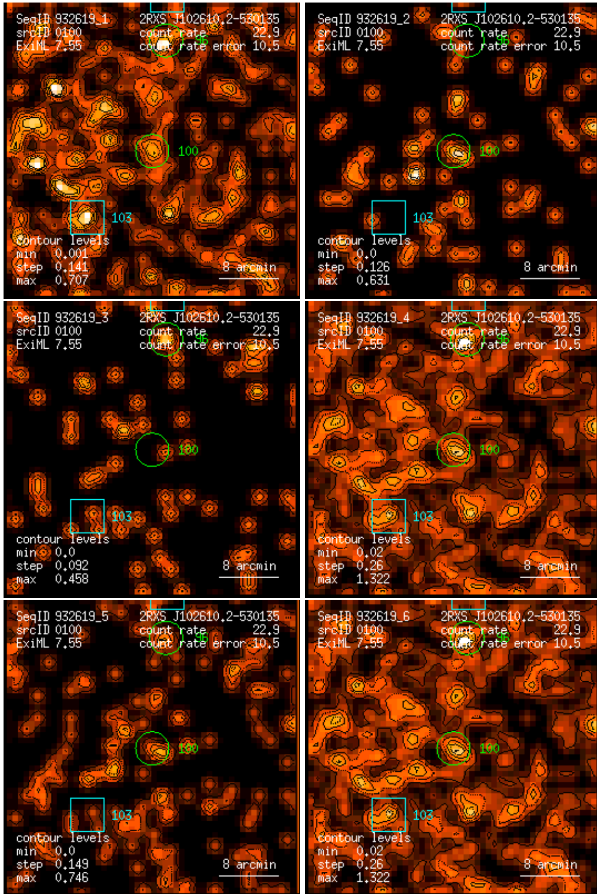
Figure 100: RASS 932619: detection 0100: band rate images, Gaussian filter: (1) PSPC channels 11 – 41, (2) 52 – 90, (3) 91 – 201, (4) 11 – 235, (5) 52 – 201, (6) 11 – 201. Broad band rates in counts/ks. Band rate contour levels in counts/ks/arcmin 2 .
