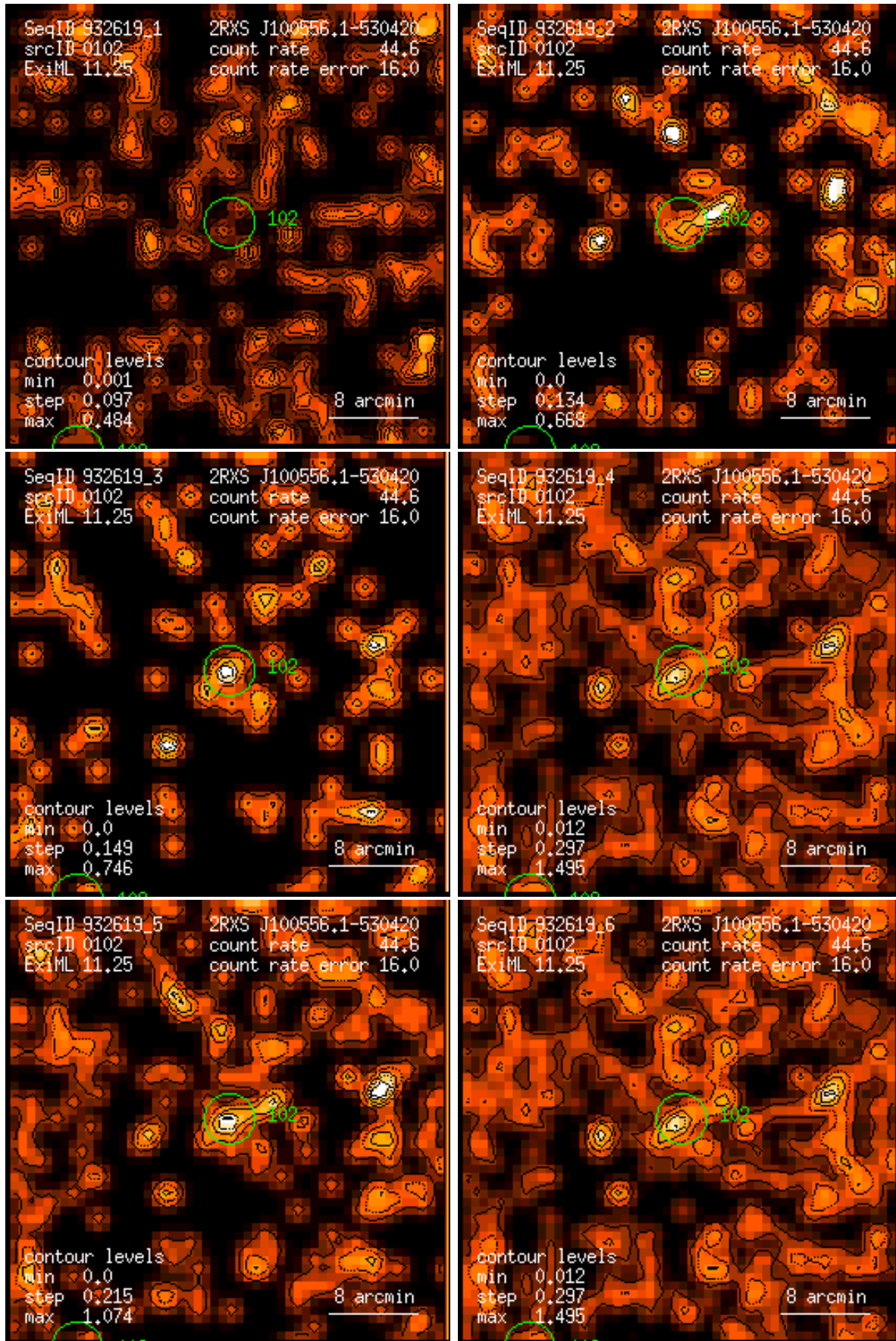
Figure 102: RASS 932619: detection 0102: band rate images, Gaussian filter: (1) PSPC channels 11 – 41, (2) 52 – 90, (3) 91 – 201, (4) 11 – 235, (5) 52 – 201, (6) 11 – 201. Broad band rates in counts/ks. Band rate contour levels in counts/ks/arcmin 2 .
