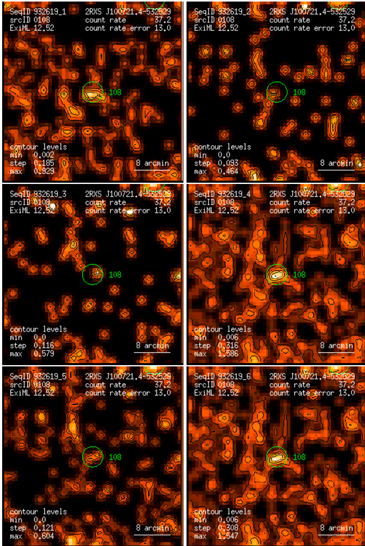
Figure 108: RASS 932619: detection 0108: band rate images, Gaussian filter: (1) PSPC channels 11 – 41, (2) 52 – 90, (3) 91 – 201, (4) 11 – 235, (5) 52 – 201, (6) 11 – 201. Broad band rates in counts/ks. Band rate contour levels in counts/ks/arcmin 2 .
