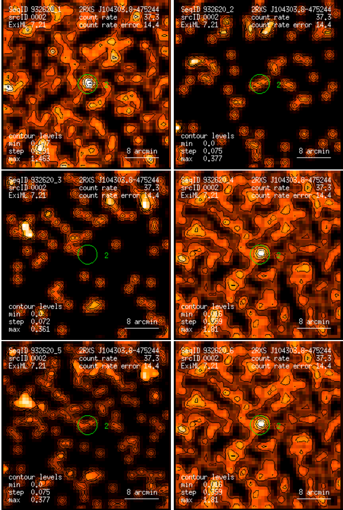
Figure 2: RASS 932620: detection 0002: band rate images, Gaussian filter: (1) PSPC channels 11 – 41, (2) 52 – 90, (3) 91 – 201, (4) 11 – 235, (5) 52 – 201, (6) 11 – 201. Broad band rates in counts/ks. Band rate contour levels in counts/ks/arcmin 2 .
