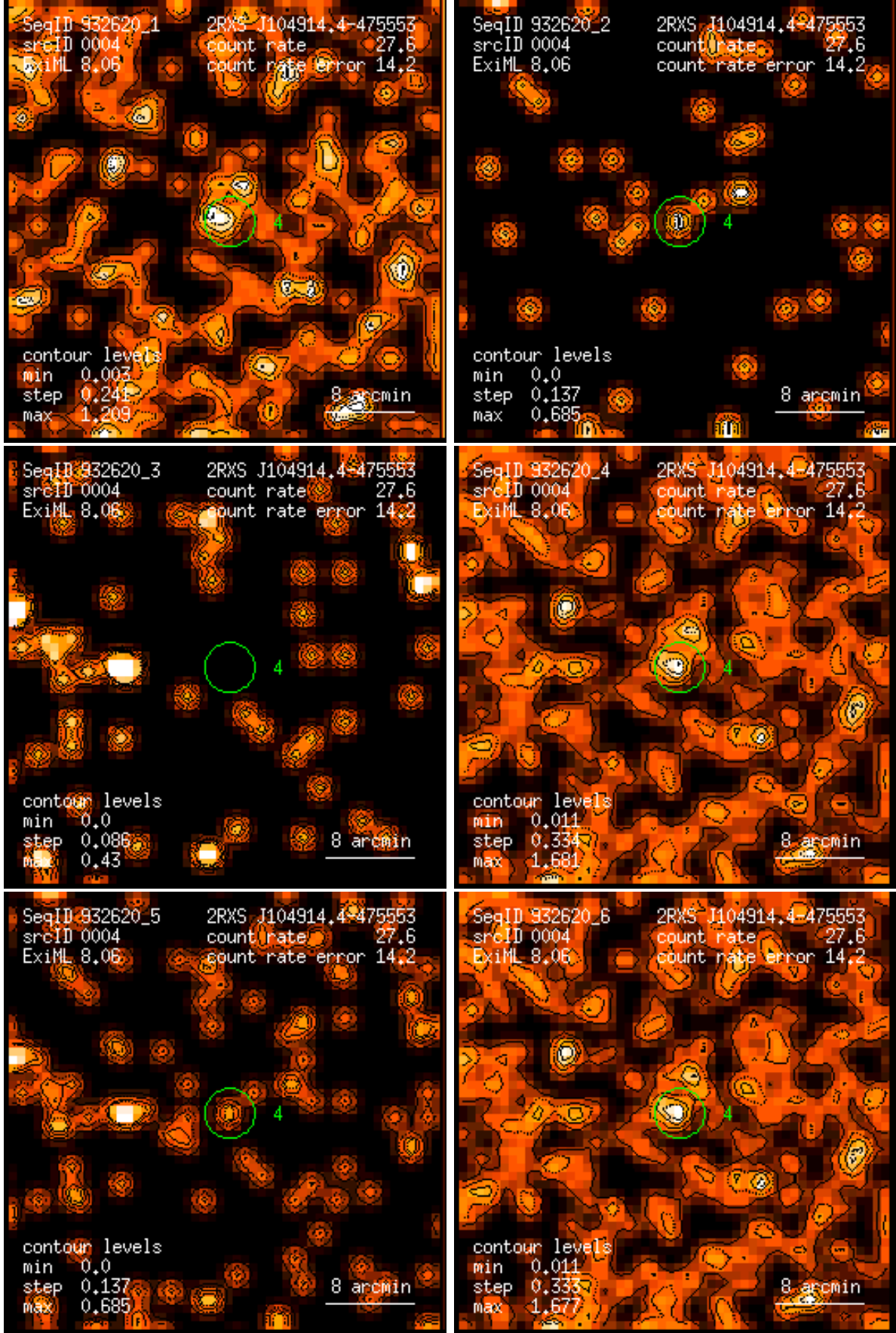
Figure 4: RASS 932620: detection 0004: band rate images, Gaussian filter: (1) PSPC channels 11 – 41, (2) 52 – 90, (3) 91 – 201, (4) 11 – 235, (5) 52 – 201, (6) 11 – 201. Broad band rates in counts/ks. Band rate contour levels in counts/ks/arcmin 2 .
