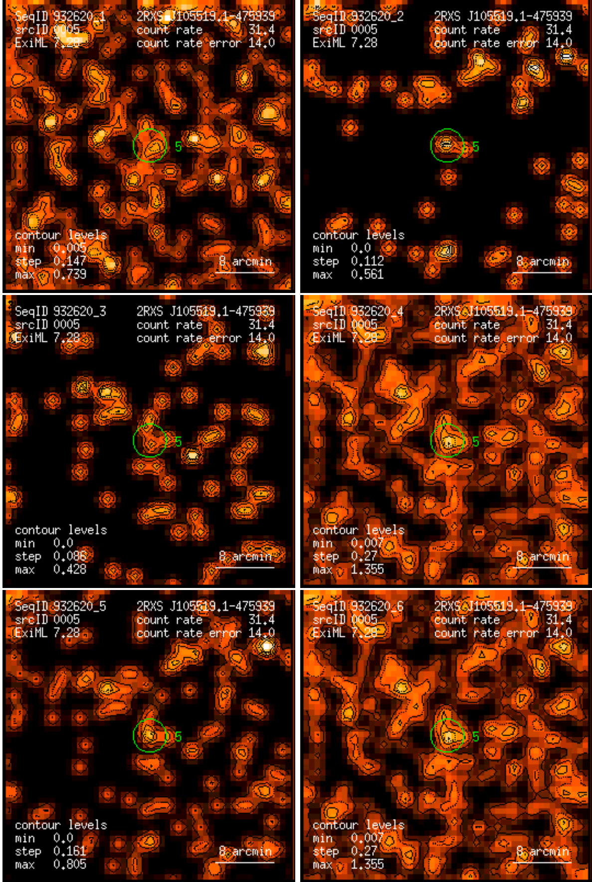
Figure 5: RASS 932620: detection 0005: band rate images, Gaussian filter: (1) PSPC channels 11 – 41, (2) 52 – 90, (3) 91 – 201, (4) 11 – 235, (5) 52 – 201, (6) 11 – 201. Broad band rates in counts/ks. Band rate contour levels in counts/ks/arcmin 2 .
