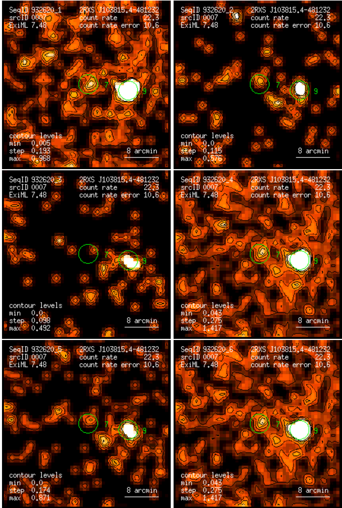
Figure 7: RASS 932620: detection 0007: band rate images, Gaussian filter: (1) PSPC channels 11 – 41, (2) 52 – 90, (3) 91 – 201, (4) 11 – 235, (5) 52 – 201, (6) 11 – 201. Broad band rates in counts/ks. Band rate contour levels in counts/ks/arcmin 2 .
