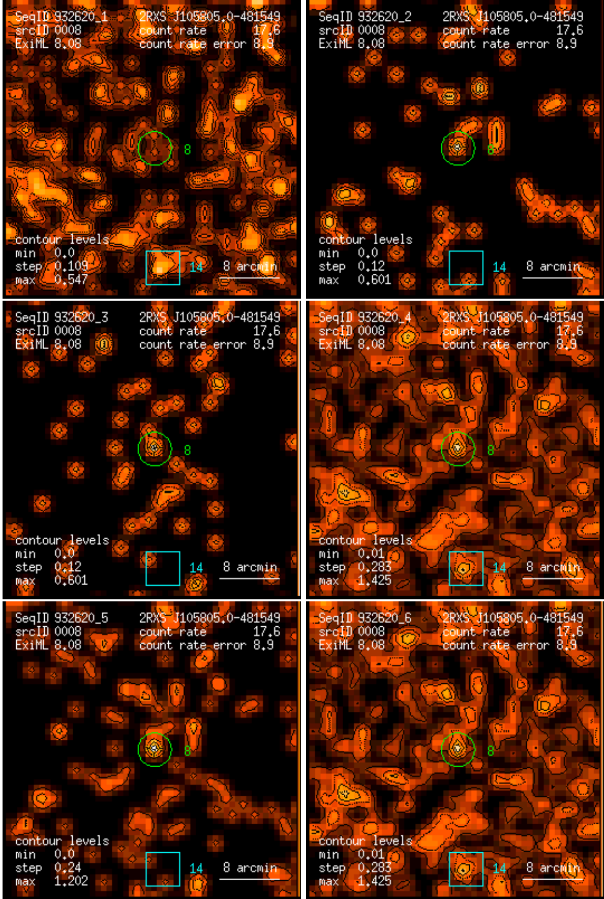
Figure 8: RASS 932620: detection 0008: band rate images, Gaussian filter: (1) PSPC channels 11 – 41, (2) 52 – 90, (3) 91 – 201, (4) 11 – 235, (5) 52 – 201, (6) 11 – 201. Broad band rates in counts/ks. Band rate contour levels in counts/ks/arcmin 2 .
