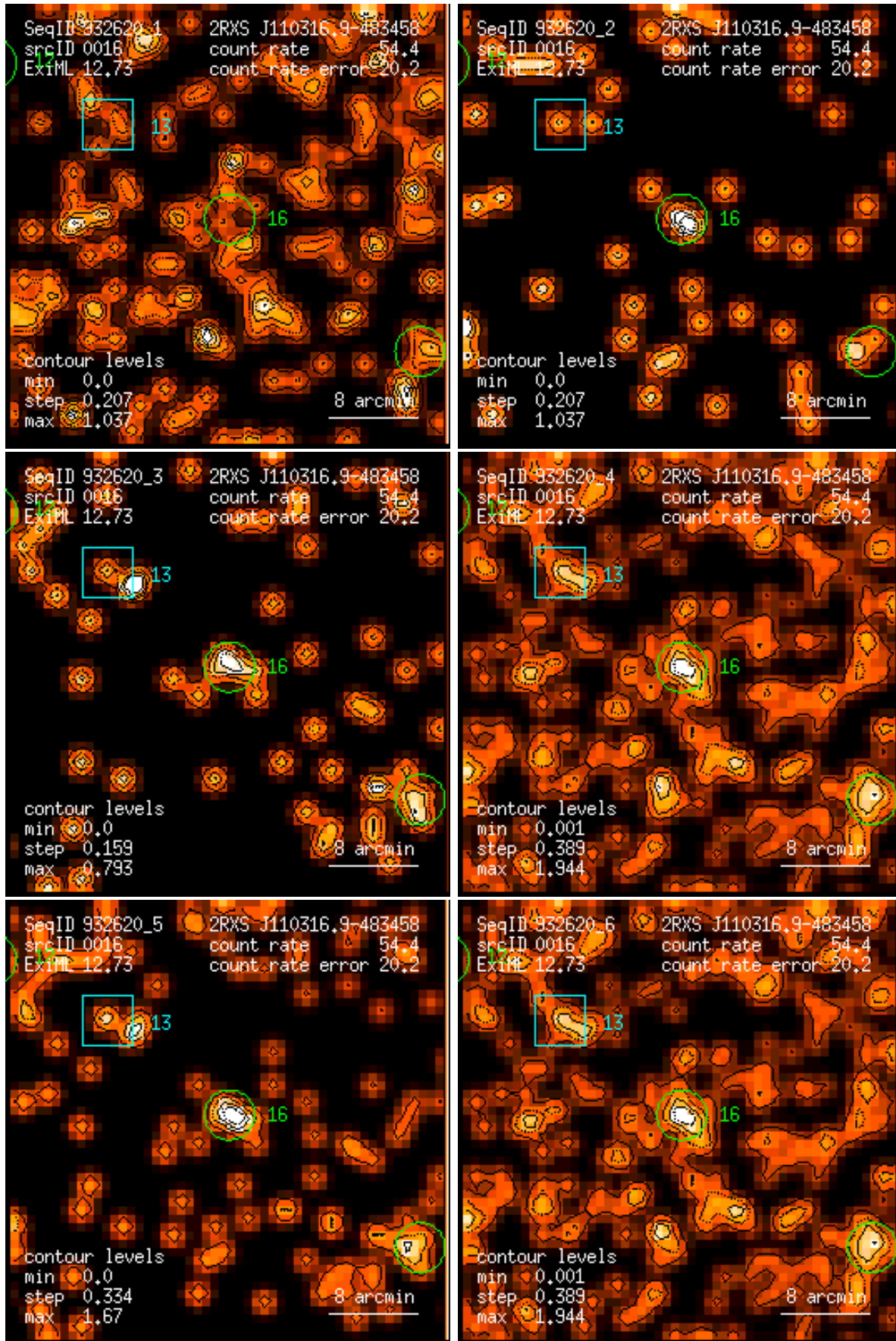
Figure 16: RASS 932620: detection 0016: band rate images, Gaussian filter: (1) PSPC channels 11 – 41, (2) 52 – 90, (3) 91 – 201, (4) 11 – 235, (5) 52 – 201, (6) 11 – 201. Broad band rates in counts/ks. Band rate contour levels in counts/ks/arcmin 2 .
