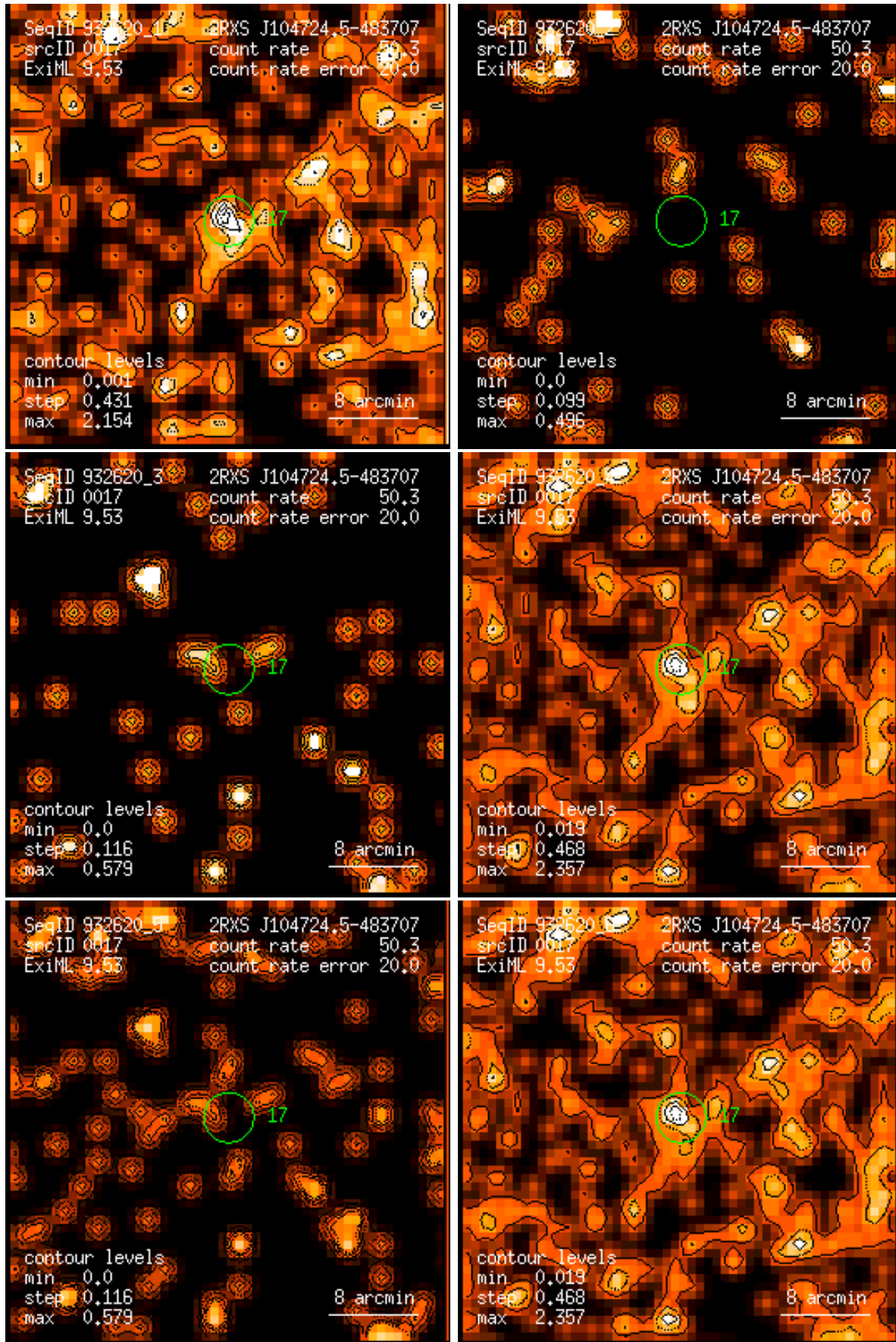
Figure 17: RASS 932620: detection 0017: band rate images, Gaussian filter: (1) PSPC channels 11 – 41, (2) 52 – 90, (3) 91 – 201, (4) 11 – 235, (5) 52 – 201, (6) 11 – 201. Broad band rates in counts/ks. Band rate contour levels in counts/ks/arcmin 2 .
