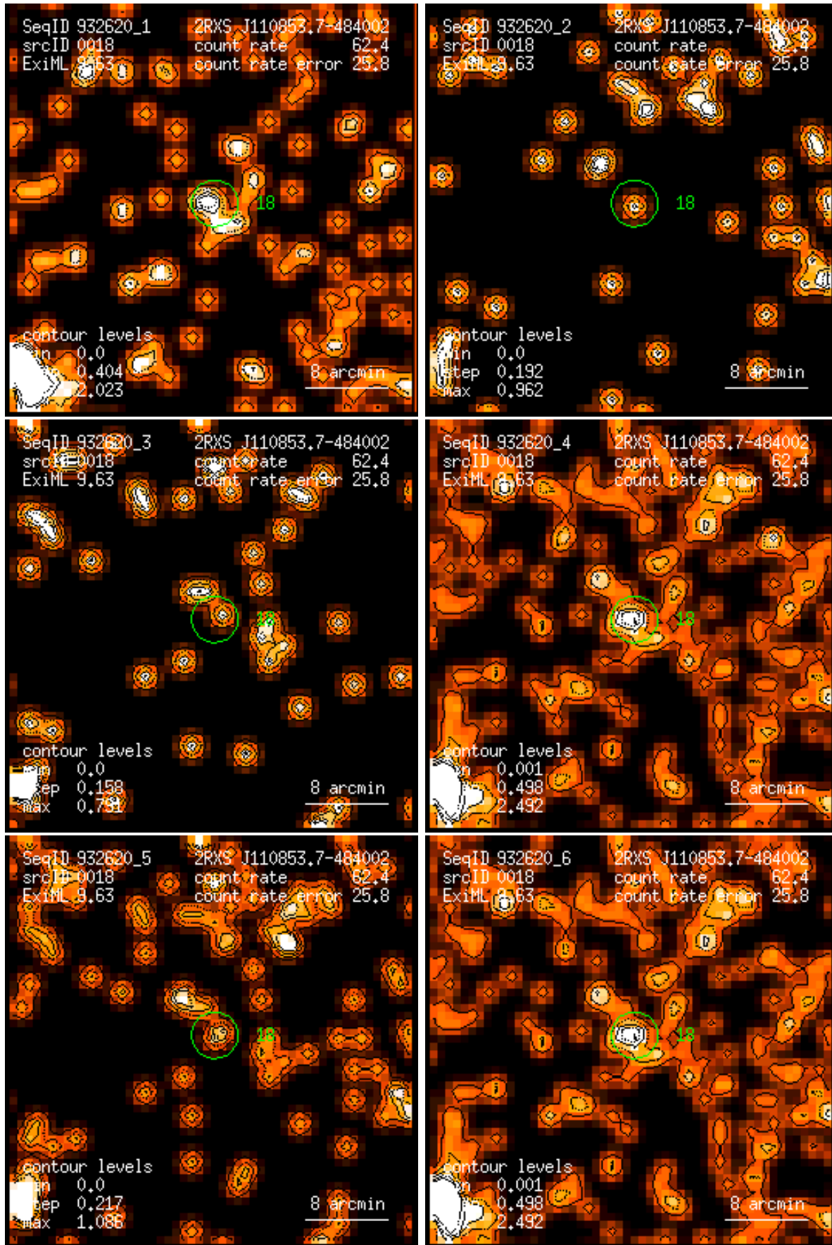
Figure 18: RASS 932620: detection 0018: band rate images, Gaussian filter: (1) PSPC channels 11 – 41, (2) 52 – 90, (3) 91 – 201, (4) 11 – 235, (5) 52 – 201, (6) 11 – 201. Broad band rates in counts/ks. Band rate contour levels in counts/ks/arcmin 2 .
