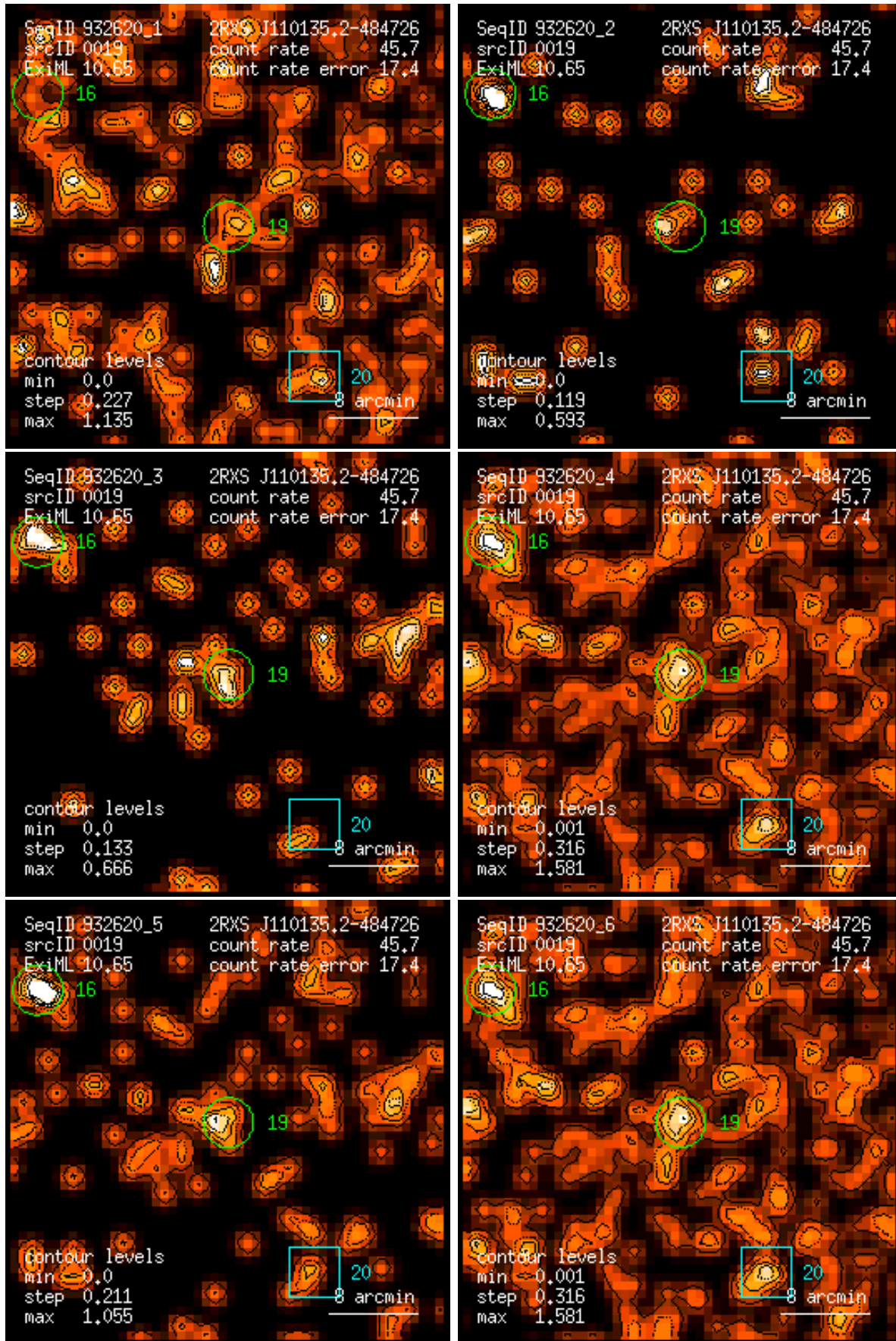
Figure 19: RASS 932620: detection 0019: band rate images, Gaussian filter: (1) PSPC channels 11 – 41, (2) 52 – 90, (3) 91 – 201, (4) 11 – 235, (5) 52 – 201, (6) 11 – 201. Broad band rates in counts/ks. Band rate contour levels in counts/ks/arcmin 2 .
