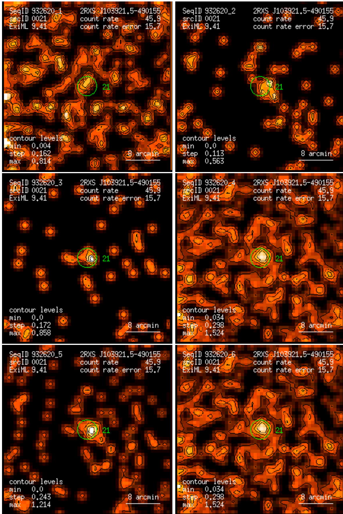
Figure 21: RASS 932620: detection 0021: band rate images, Gaussian filter: (1) PSPC channels 11 – 41, (2) 52 – 90, (3) 91 – 201, (4) 11 – 235, (5) 52 – 201, (6) 11 – 201. Broad band rates in counts/ks. Band rate contour levels in counts/ks/arcmin 2 .
