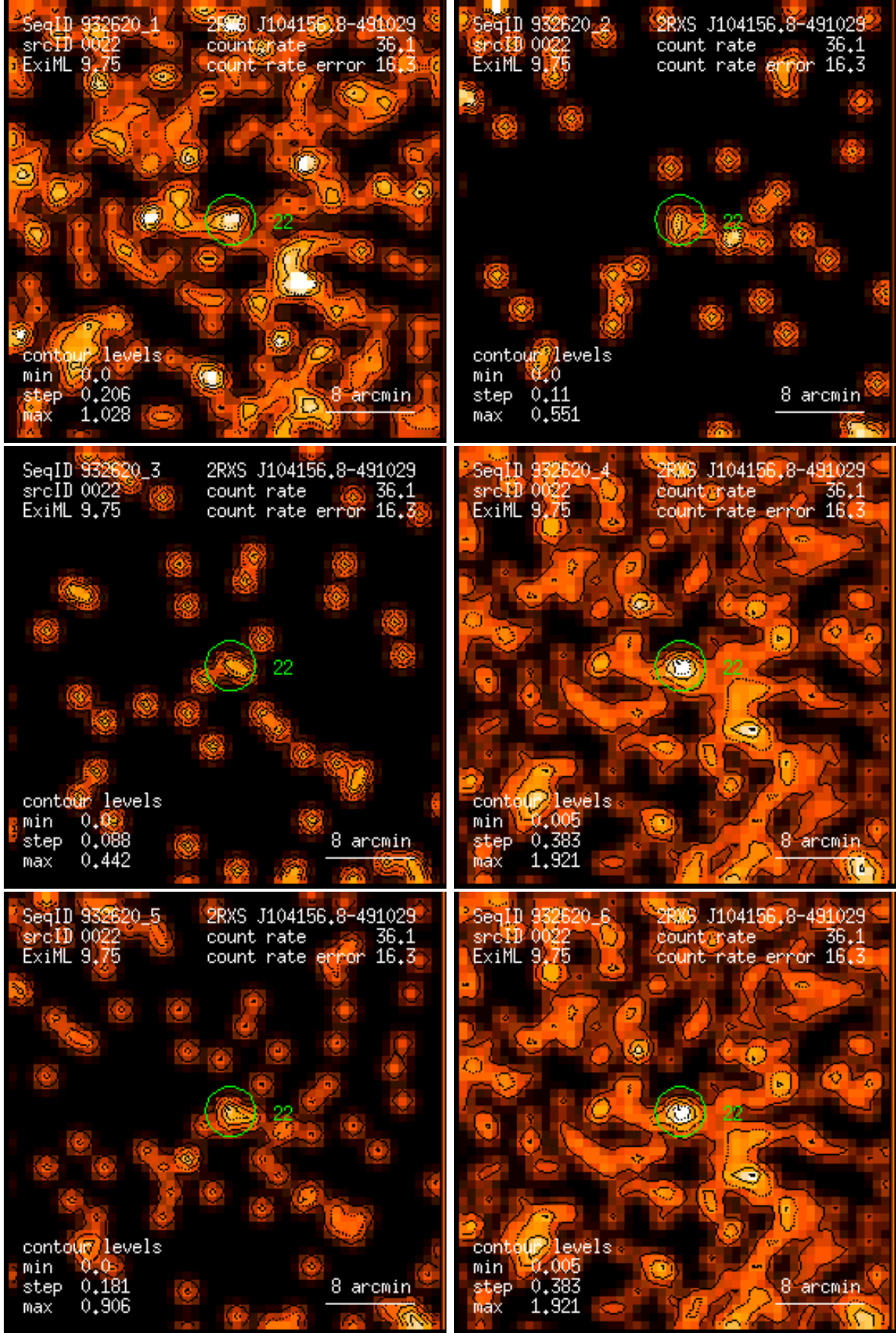
Figure 22: RASS 932620: detection 0022: band rate images, Gaussian filter: (1) PSPC channels 11 – 41, (2) 52 – 90, (3) 91 – 201, (4) 11 – 235, (5) 52 – 201, (6) 11 – 201. Broad band rates in counts/ks. Band rate contour levels in counts/ks/arcmin 2 .
