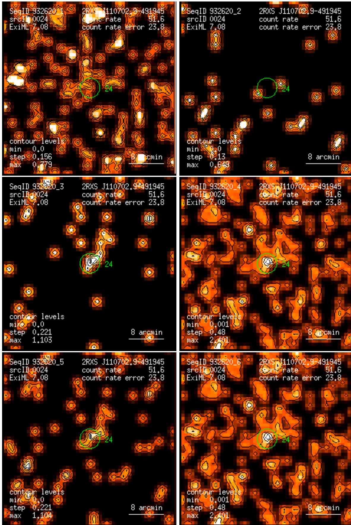
Figure 24: RASS 932620: detection 0024: band rate images, Gaussian filter: (1) PSPC channels 11 – 41, (2) 52 – 90, (3) 91 – 201, (4) 11 – 235, (5) 52 – 201, (6) 11 – 201. Broad band rates in counts/ks. Band rate contour levels in counts/ks/arcmin 2 .
