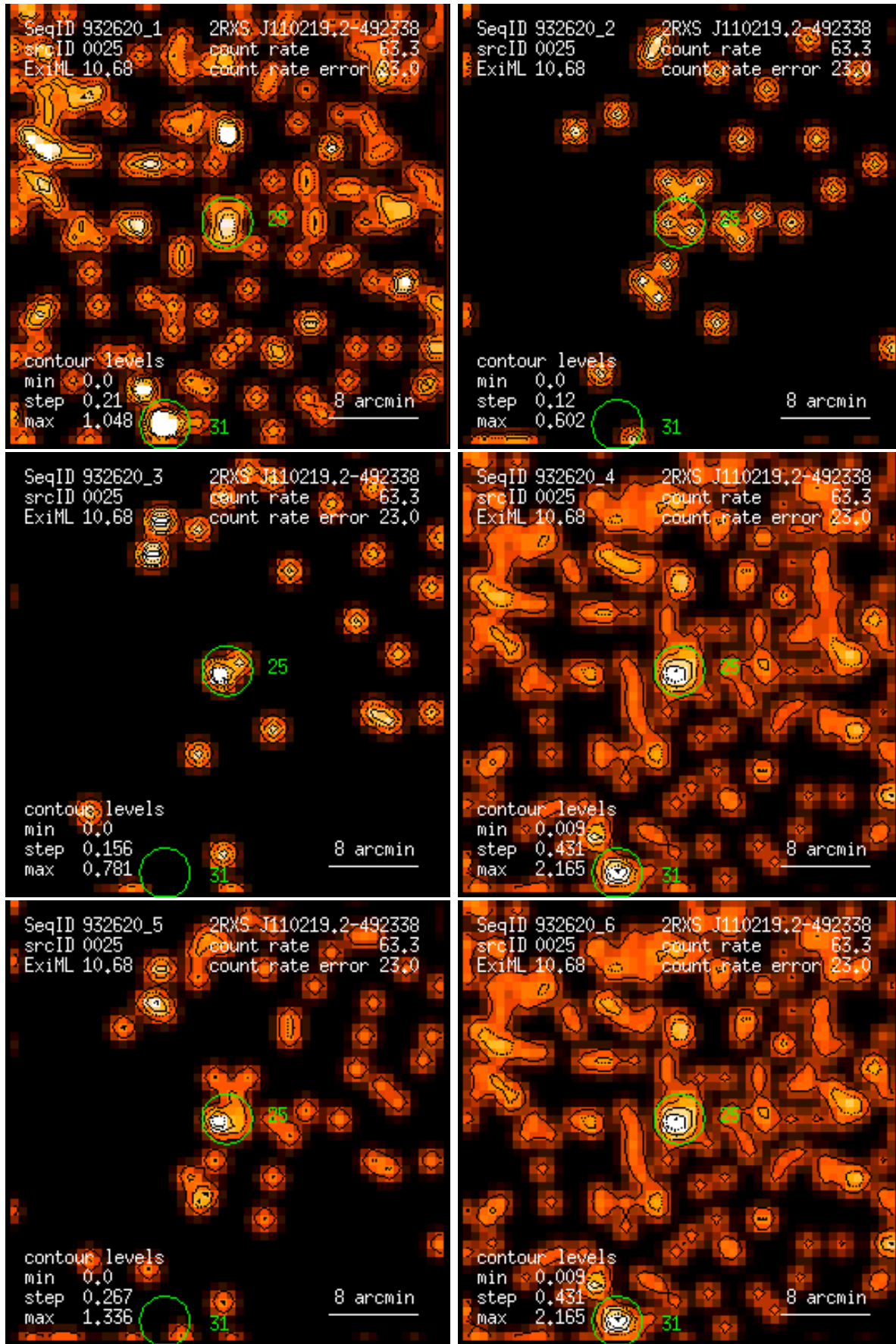
Figure 25: RASS 932620: detection 0025: band rate images, Gaussian filter: (1) PSPC channels 11 – 41, (2) 52 – 90, (3) 91 – 201, (4) 11 – 235, (5) 52 – 201, (6) 11 – 201. Broad band rates in counts/ks. Band rate contour levels in counts/ks/arcmin 2 .
