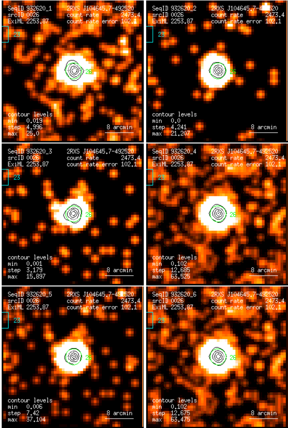
Figure 26: RASS 932620: detection 0026: band rate images, Gaussian filter: (1) PSPC channels 11 – 41, (2) 52 – 90, (3) 91 – 201, (4) 11 – 235, (5) 52 – 201, (6) 11 – 201. Broad band rates in counts/ks. Band rate contour levels in counts/ks/arcmin 2 .
