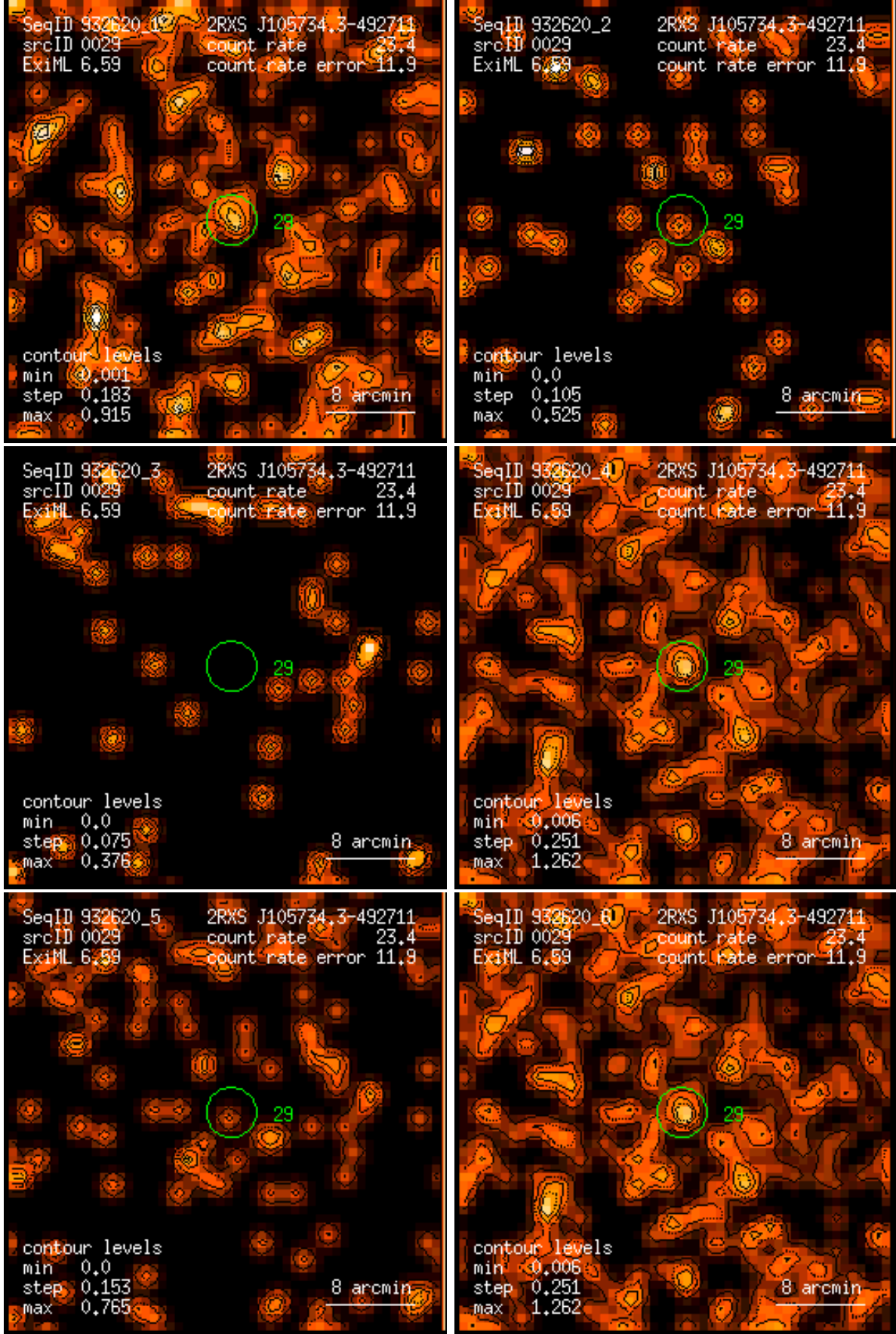
Figure 29: RASS 932620: detection 0029: band rate images, Gaussian filter: (1) PSPC channels 11 – 41, (2) 52 – 90, (3) 91 – 201, (4) 11 – 235, (5) 52 – 201, (6) 11 – 201. Broad band rates in counts/ks. Band rate contour levels in counts/ks/arcmin 2 .
