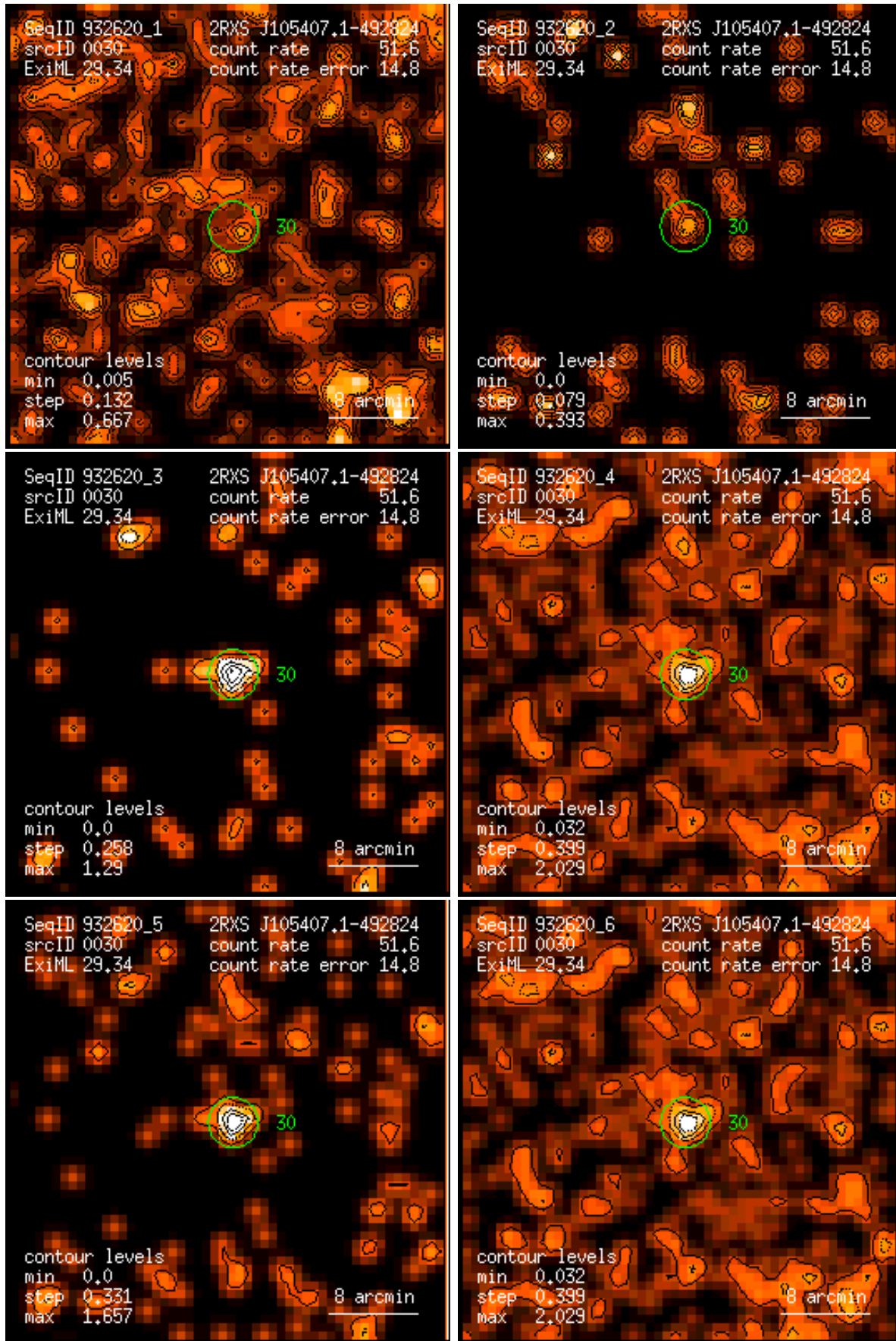
Figure 30: RASS 932620: detection 0030: band rate images, Gaussian filter: (1) PSPC channels 11 – 41, (2) 52 – 90, (3) 91 – 201, (4) 11 – 235, (5) 52 – 201, (6) 11 – 201. Broad band rates in counts/ks. Band rate contour levels in counts/ks/arcmin 2 .
