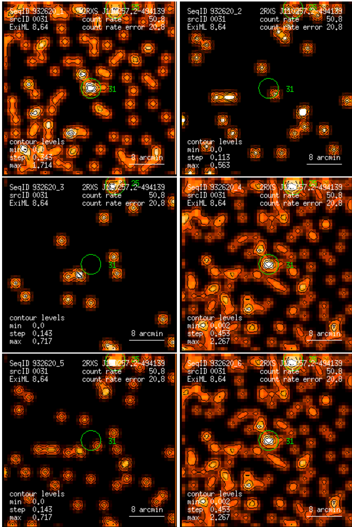
Figure 31: RASS 932620: detection 0031: band rate images, Gaussian filter: (1) PSPC channels 11 – 41, (2) 52 – 90, (3) 91 – 201, (4) 11 – 235, (5) 52 – 201, (6) 11 – 201. Broad band rates in counts/ks. Band rate contour levels in counts/ks/arcmin 2 .
