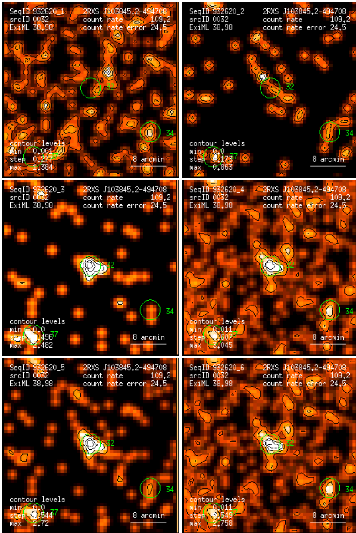
Figure 32: RASS 932620: detection 0032: band rate images, Gaussian filter: (1) PSPC channels 11 – 41, (2) 52 – 90, (3) 91 – 201, (4) 11 – 235, (5) 52 – 201, (6) 11 – 201. Broad band rates in counts/ks. Band rate contour levels in counts/ks/arcmin 2 .
