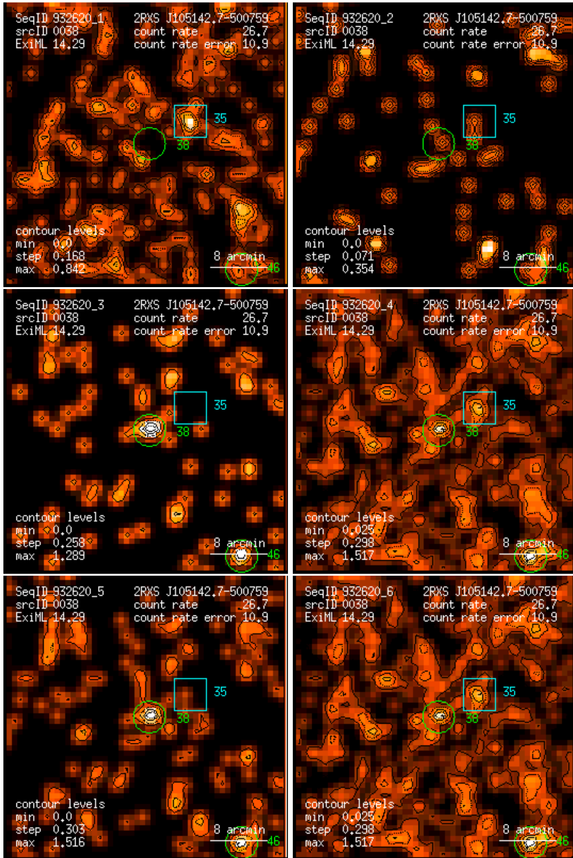
Figure 38: RASS 932620: detection 0038: band rate images, Gaussian filter: (1) PSPC channels 11 – 41, (2) 52 – 90, (3) 91 – 201, (4) 11 – 235, (5) 52 – 201, (6) 11 – 201. Broad band rates in counts/ks. Band rate contour levels in counts/ks/arcmin 2 .
