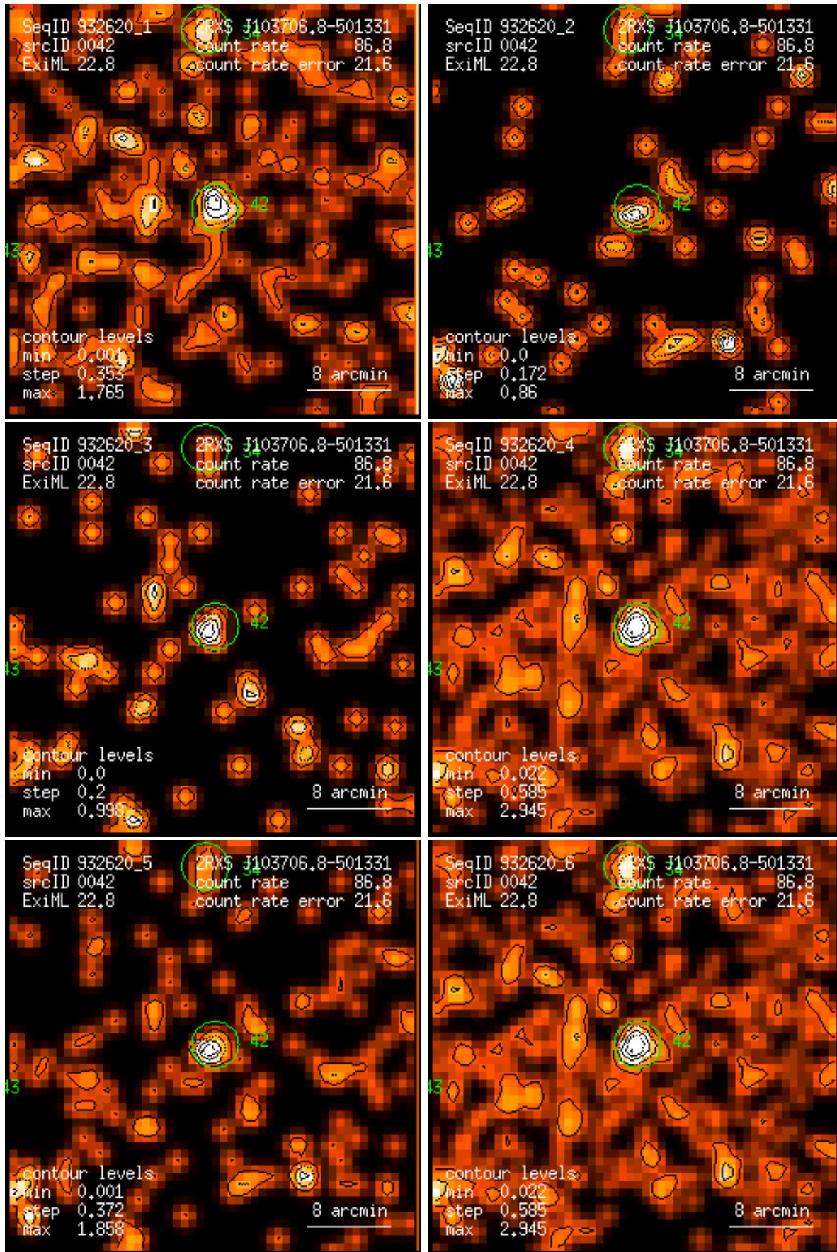
Figure 42: RASS 932620: detection 0042: band rate images, Gaussian filter: (1) PSPC channels 11 – 41, (2) 52 – 90, (3) 91 – 201, (4) 11 – 235, (5) 52 – 201, (6) 11 – 201. Broad band rates in counts/ks. Band rate contour levels in counts/ks/arcmin 2 .
