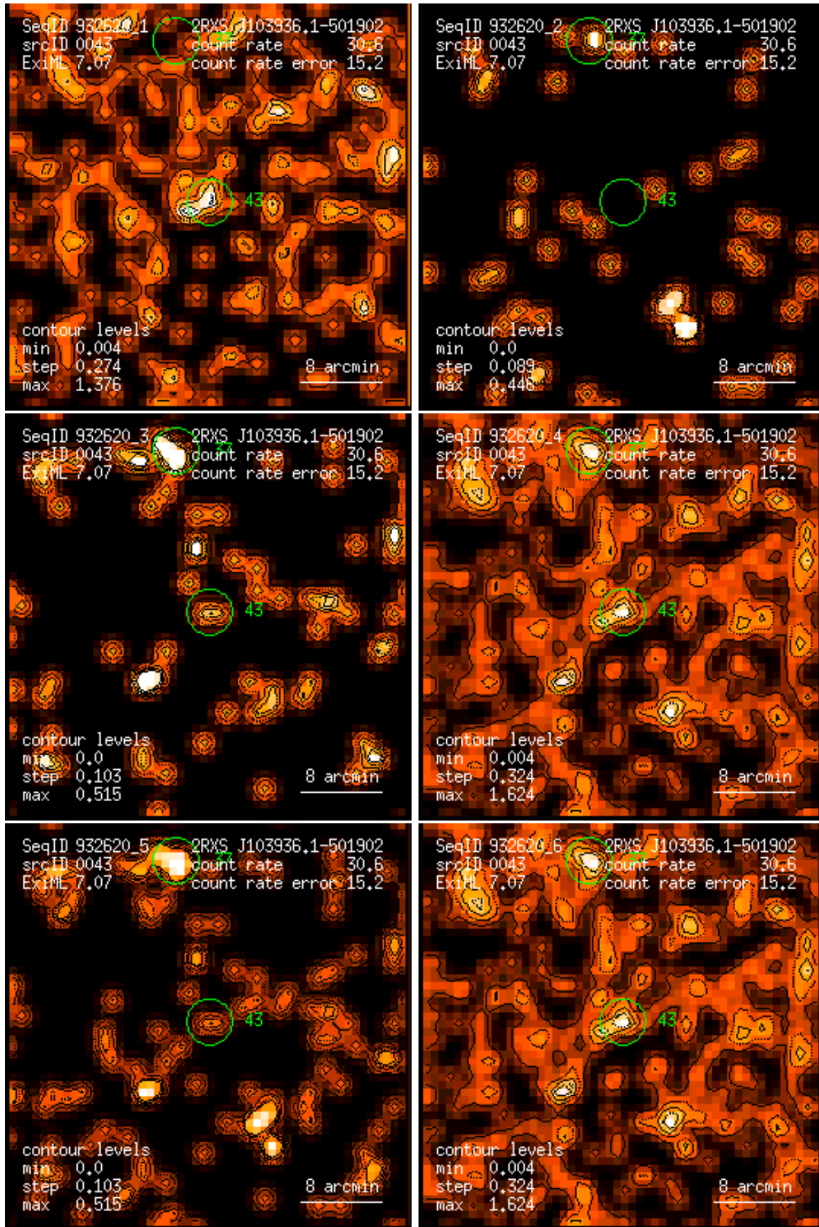
Figure 43: RASS 932620: detection 0043: band rate images, Gaussian filter: (1) PSPC channels 11 – 41, (2) 52 – 90, (3) 91 – 201, (4) 11 – 235, (5) 52 – 201, (6) 11 – 201. Broad band rates in counts/ks. Band rate contour levels in counts/ks/arcmin 2 .
