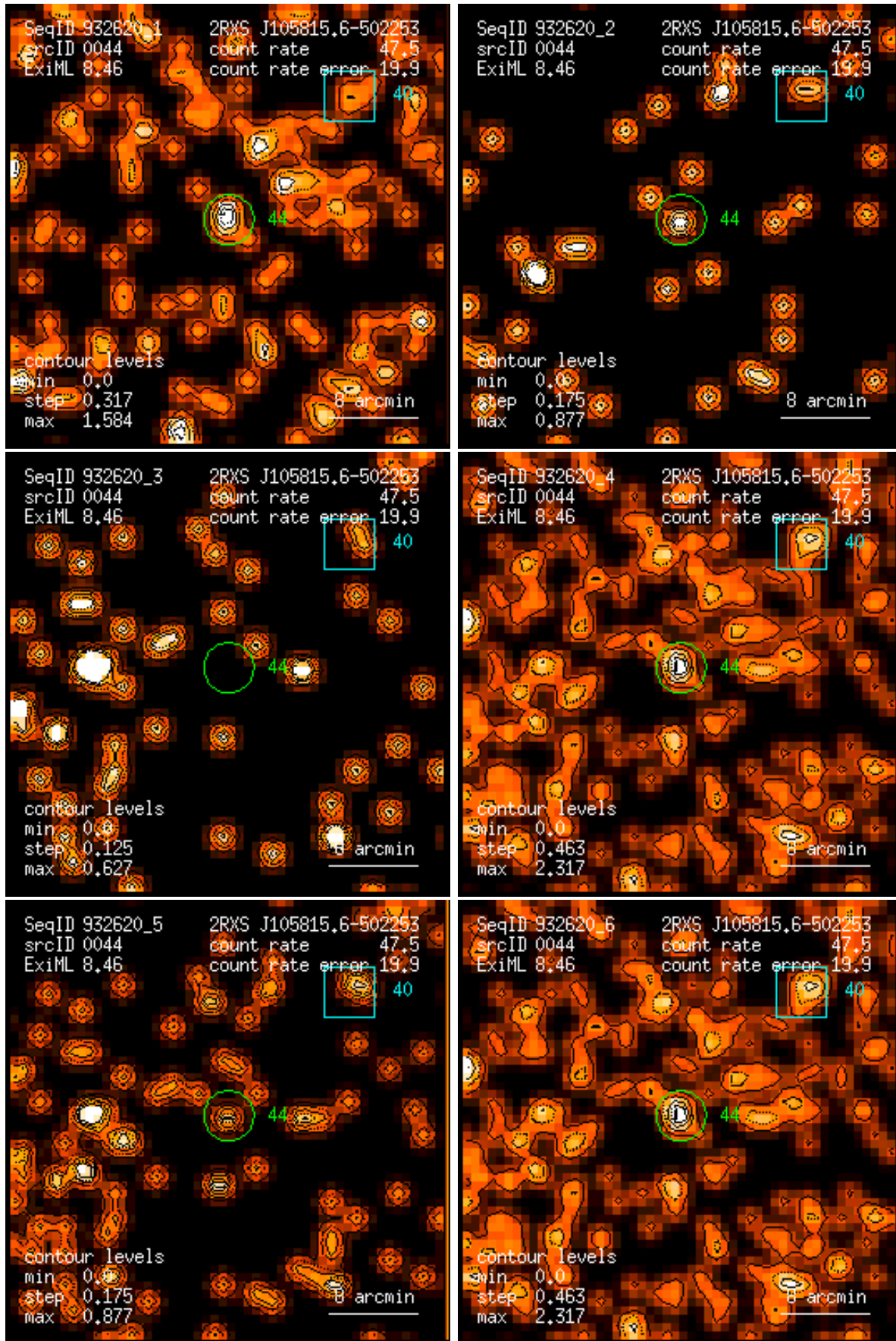
Figure 44: RASS 932620: detection 0044: band rate images, Gaussian filter: (1) PSPC channels 11 – 41, (2) 52 – 90, (3) 91 – 201, (4) 11 – 235, (5) 52 – 201, (6) 11 – 201. Broad band rates in counts/ks. Band rate contour levels in counts/ks/arcmin 2 .
