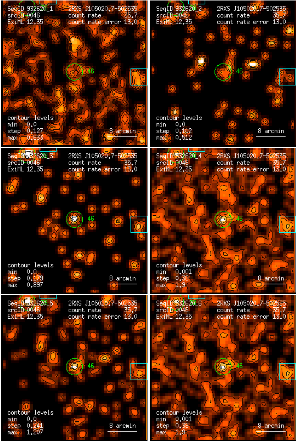
Figure 46: RASS 932620: detection 0046: band rate images, Gaussian filter: (1) PSPC channels 11 – 41, (2) 52 – 90, (3) 91 – 201, (4) 11 – 235, (5) 52 – 201, (6) 11 – 201. Broad band rates in counts/ks. Band rate contour levels in counts/ks/arcmin 2 .
