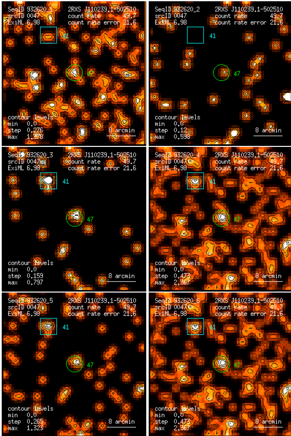
Figure 47: RASS 932620: detection 0047: band rate images, Gaussian filter: (1) PSPC channels 11 – 41, (2) 52 – 90, (3) 91 – 201, (4) 11 – 235, (5) 52 – 201, (6) 11 – 201. Broad band rates in counts/ks. Band rate contour levels in counts/ks/arcmin 2 .
