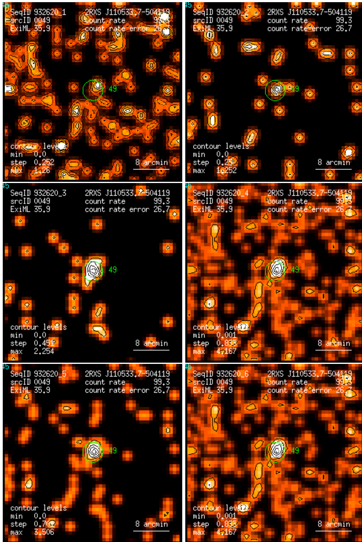
Figure 49: RASS 932620: detection 0049: band rate images, Gaussian filter: (1) PSPC channels 11 – 41, (2) 52 – 90, (3) 91 – 201, (4) 11 – 235, (5) 52 – 201, (6) 11 – 201. Broad band rates in counts/ks. Band rate contour levels in counts/ks/arcmin 2 .
