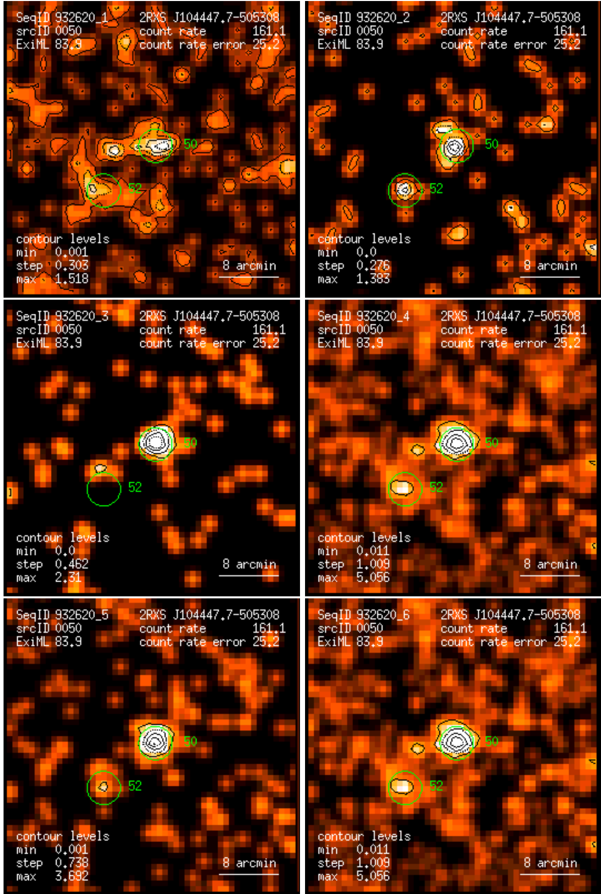
Figure 50: RASS 932620: detection 0050: band rate images, Gaussian filter: (1) PSPC channels 11 – 41, (2) 52 – 90, (3) 91 – 201, (4) 11 – 235, (5) 52 – 201, (6) 11 – 201. Broad band rates in counts/ks. Band rate contour levels in counts/ks/arcmin 2 .
