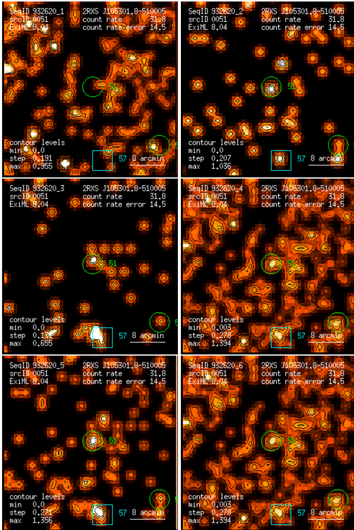
Figure 51: RASS 932620: detection 0051: band rate images, Gaussian filter: (1) PSPC channels 11 – 41, (2) 52 – 90, (3) 91 – 201, (4) 11 – 235, (5) 52 – 201, (6) 11 – 201. Broad band rates in counts/ks. Band rate contour levels in counts/ks/arcmin 2 .
