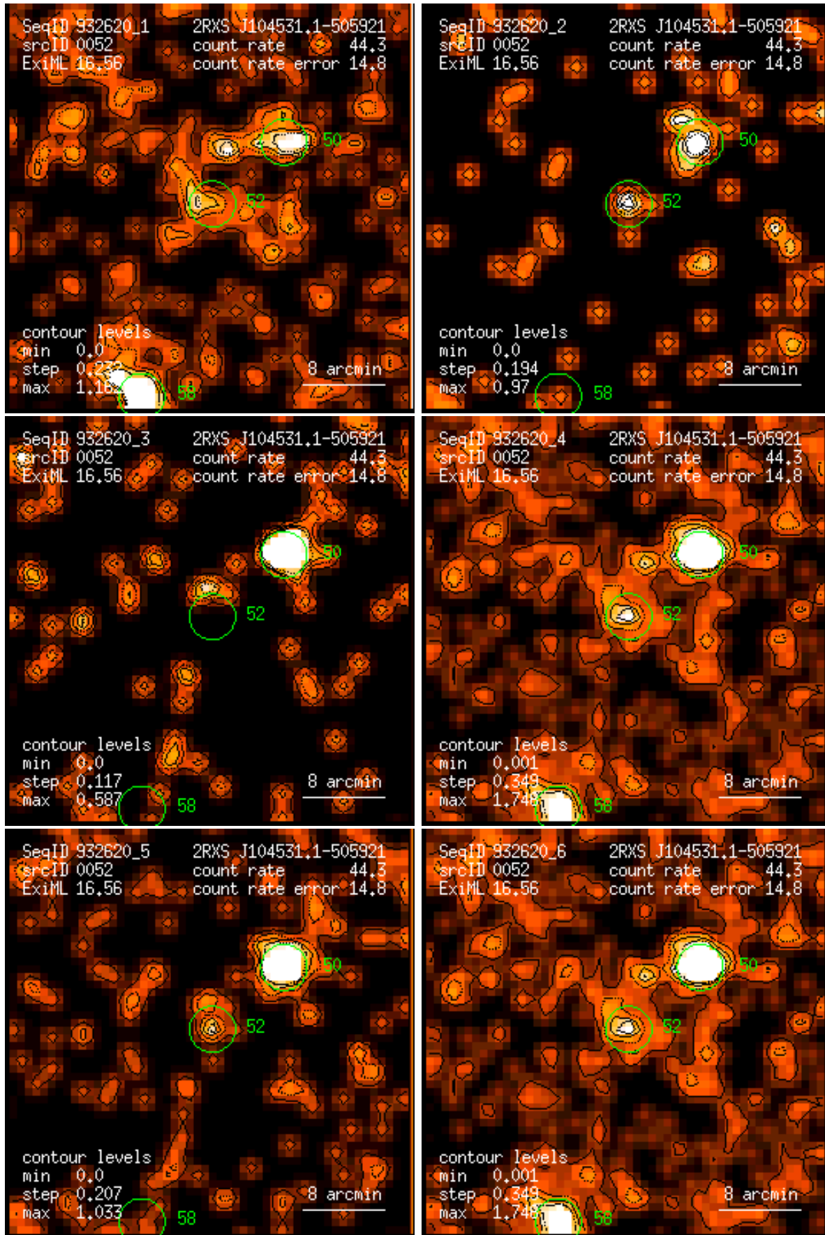
Figure 52: RASS 932620: detection 0052: band rate images, Gaussian filter: (1) PSPC channels 11 – 41, (2) 52 – 90, (3) 91 – 201, (4) 11 – 235, (5) 52 – 201, (6) 11 – 201. Broad band rates in counts/ks. Band rate contour levels in counts/ks/arcmin 2 .
