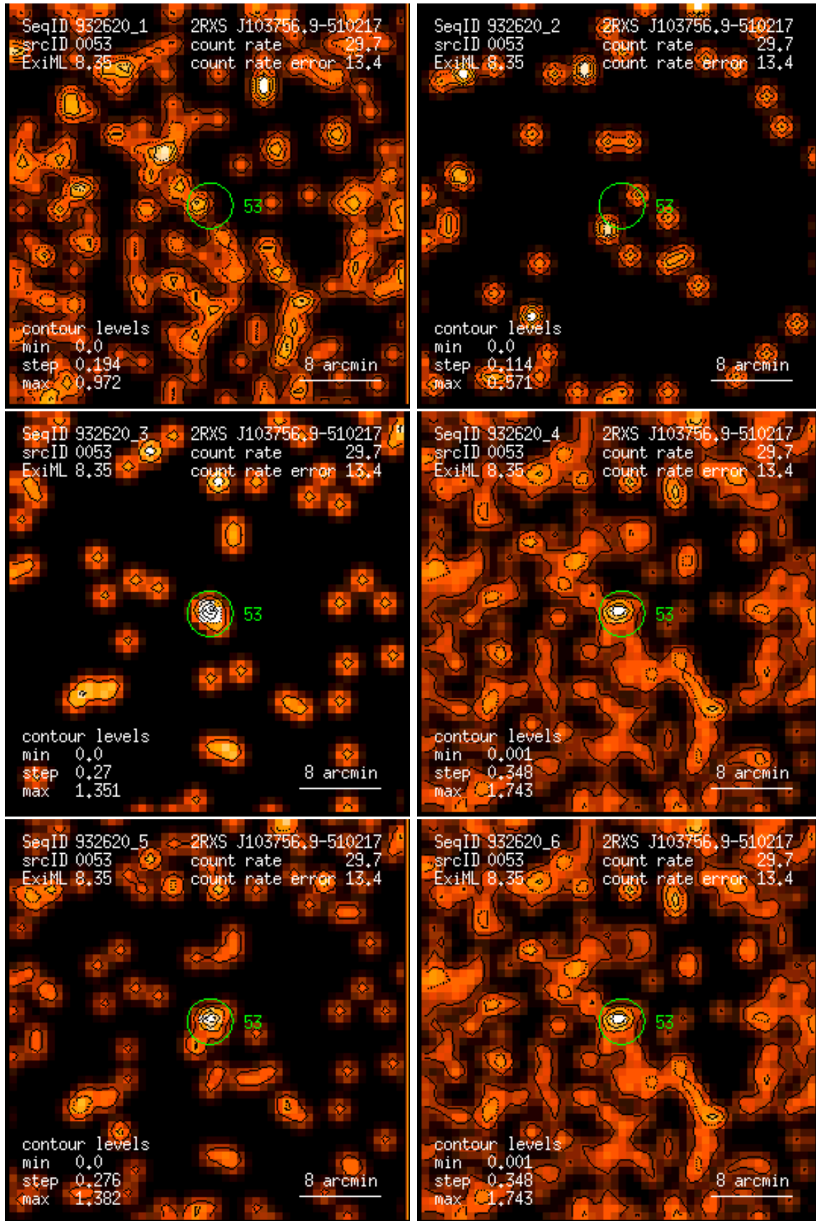
Figure 53: RASS 932620: detection 0053: band rate images, Gaussian filter: (1) PSPC channels 11 – 41, (2) 52 – 90, (3) 91 – 201, (4) 11 – 235, (5) 52 – 201, (6) 11 – 201. Broad band rates in counts/ks. Band rate contour levels in counts/ks/arcmin 2 .
