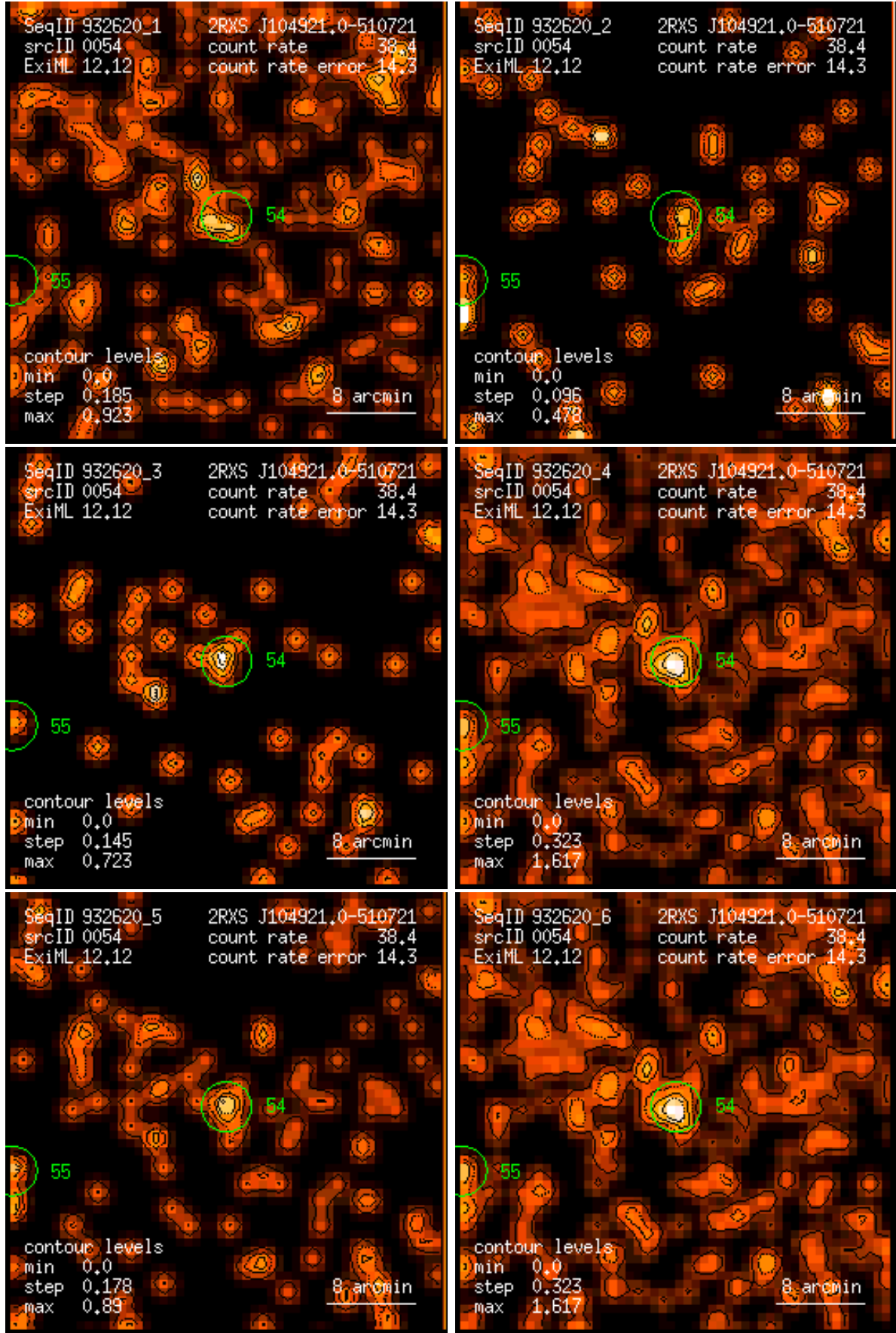
Figure 54: RASS 932620: detection 0054: band rate images, Gaussian filter: (1) PSPC channels 11 – 41, (2) 52 – 90, (3) 91 – 201, (4) 11 – 235, (5) 52 – 201, (6) 11 – 201. Broad band rates in counts/ks. Band rate contour levels in counts/ks/arcmin 2 .
