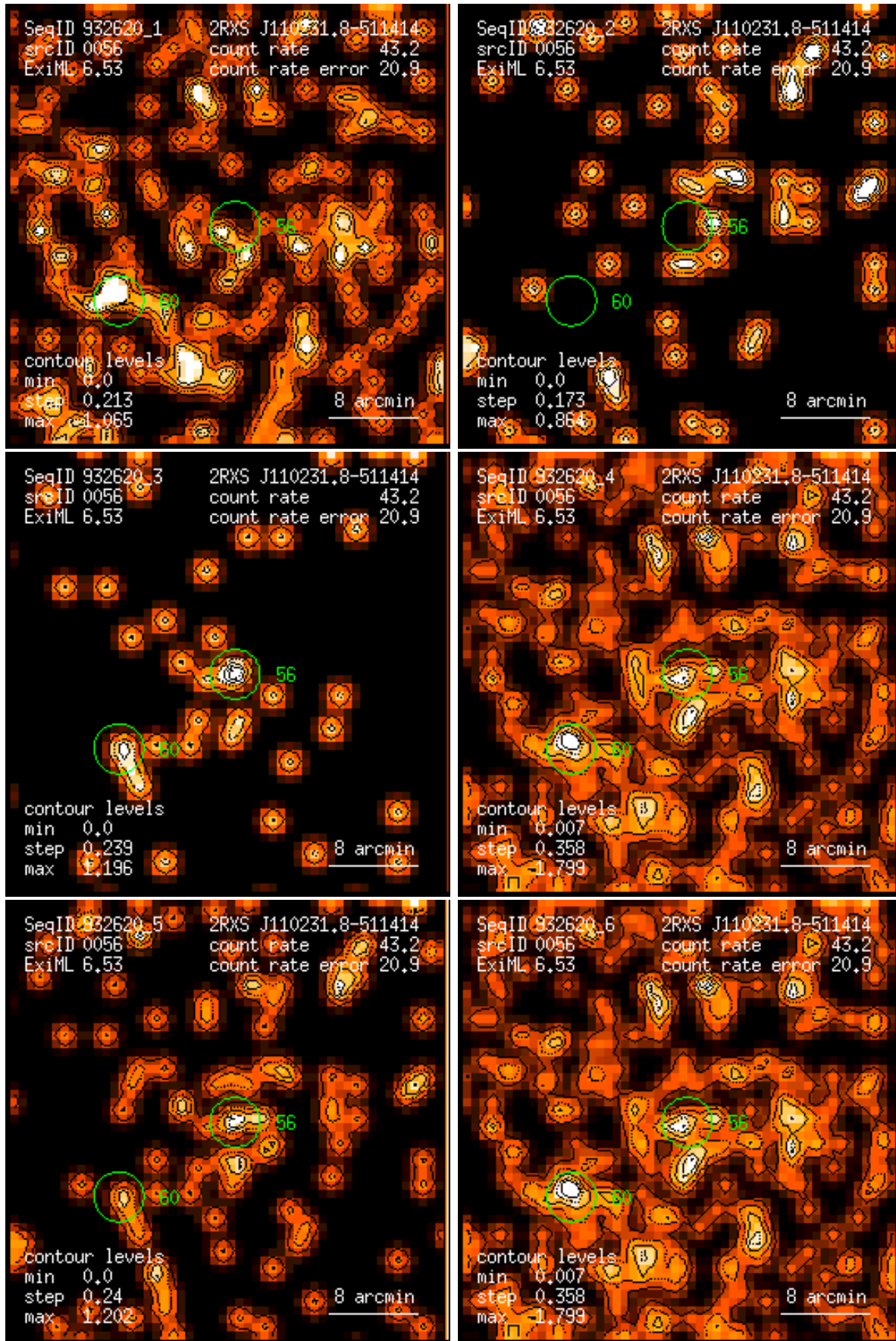
Figure 56: RASS 932620: detection 0056: band rate images, Gaussian filter: (1) PSPC channels 11 – 41, (2) 52 – 90, (3) 91 – 201, (4) 11 – 235, (5) 52 – 201, (6) 11 – 201. Broad band rates in counts/ks. Band rate contour levels in counts/ks/arcmin 2 .
