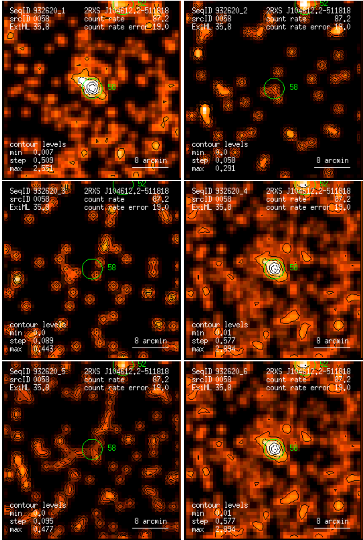
Figure 58: RASS 932620: detection 0058: band rate images, Gaussian filter: (1) PSPC channels 11 – 41, (2) 52 – 90, (3) 91 – 201, (4) 11 – 235, (5) 52 – 201, (6) 11 – 201. Broad band rates in counts/ks. Band rate contour levels in counts/ks/arcmin 2 .
