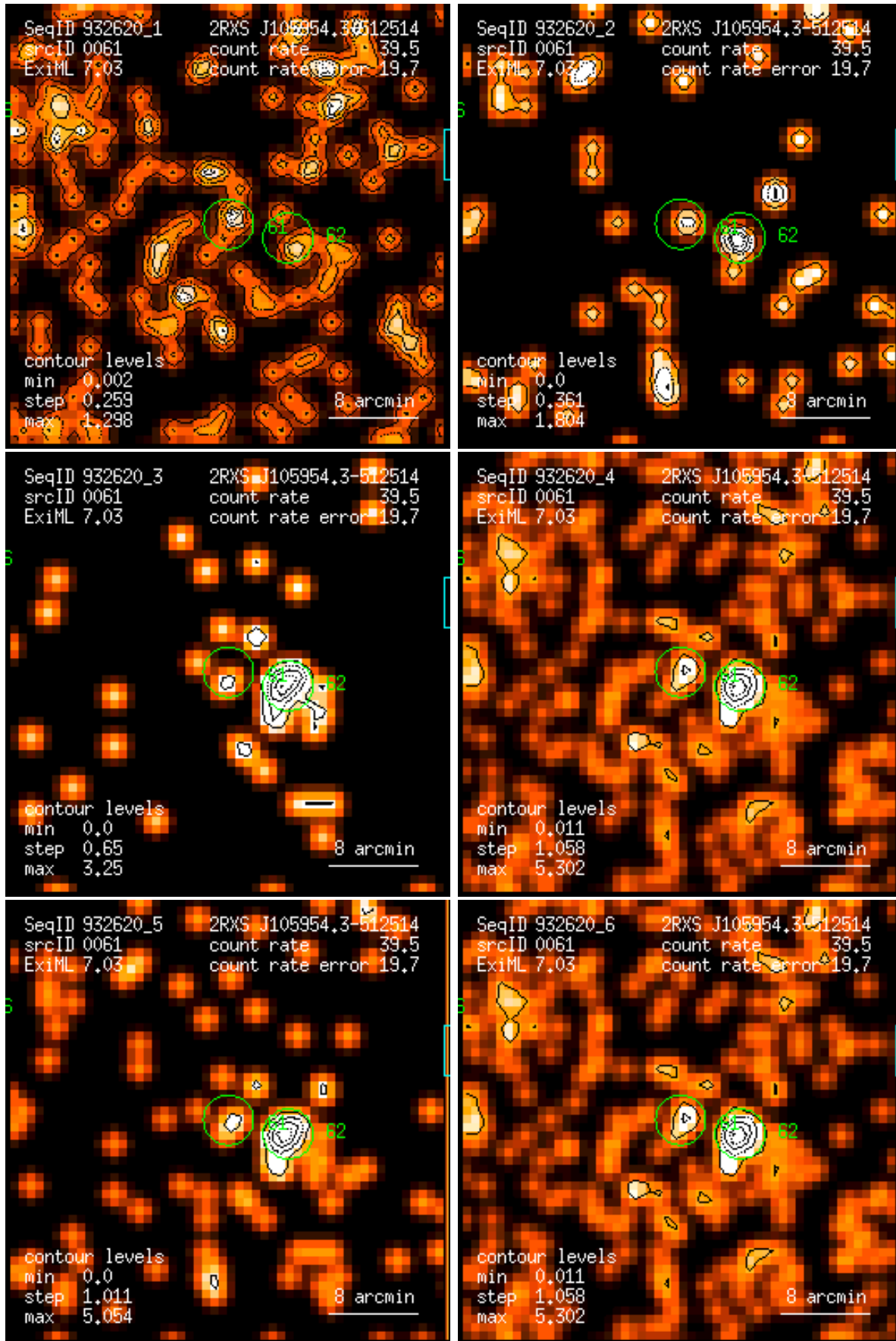
Figure 61: RASS 932620: detection 0061: band rate images, Gaussian filter: (1) PSPC channels 11 – 41, (2) 52 – 90, (3) 91 – 201, (4) 11 – 235, (5) 52 – 201, (6) 11 – 201. Broad band rates in counts/ks. Band rate contour levels in counts/ks/arcmin 2 .
